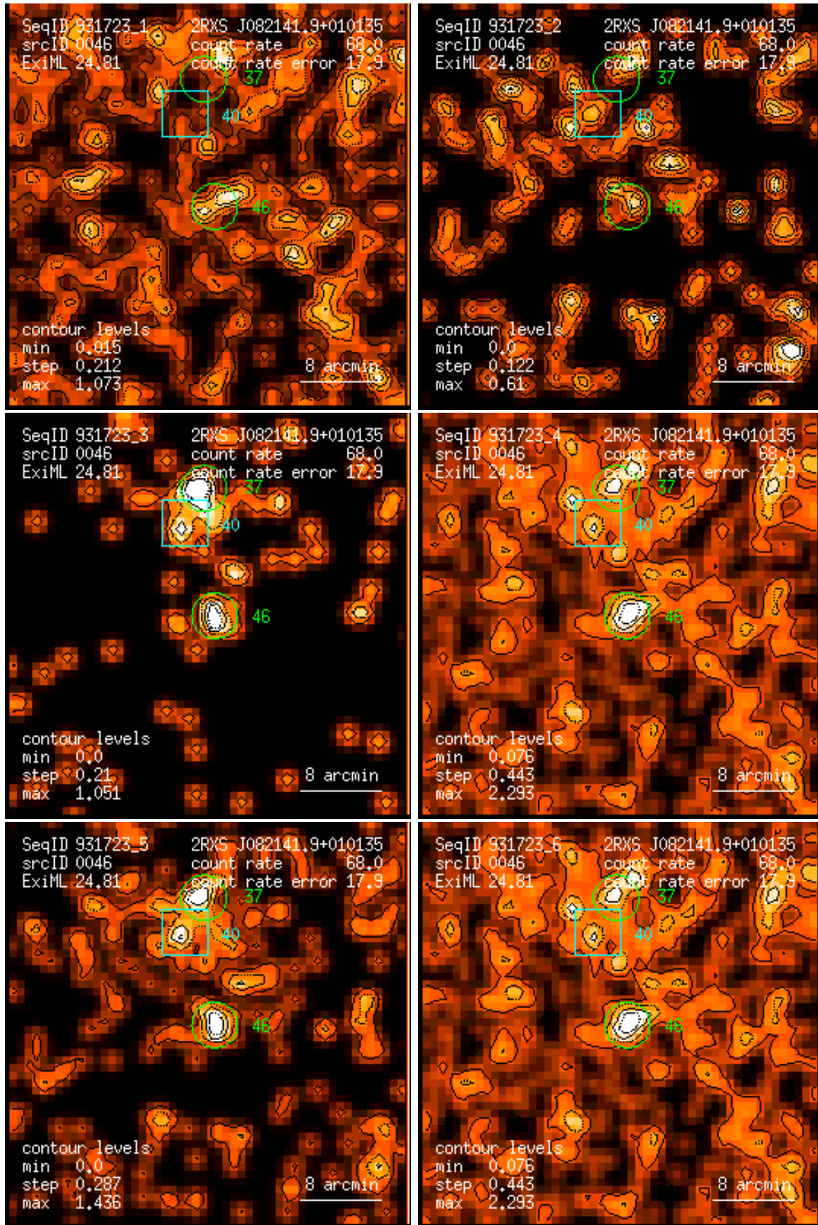
Figure 46: RASS 931723: detection 0046: band rate images, Gaussian filter: (1) PSPC channels 11 – 41, (2) 52 – 90, (3) 91 – 201, (4) 11 – 235, (5) 52 – 201, (6) 11 – 201. Broad band rates in counts/ks. Band rate contour levels in counts/ks/arcmin 2 .
