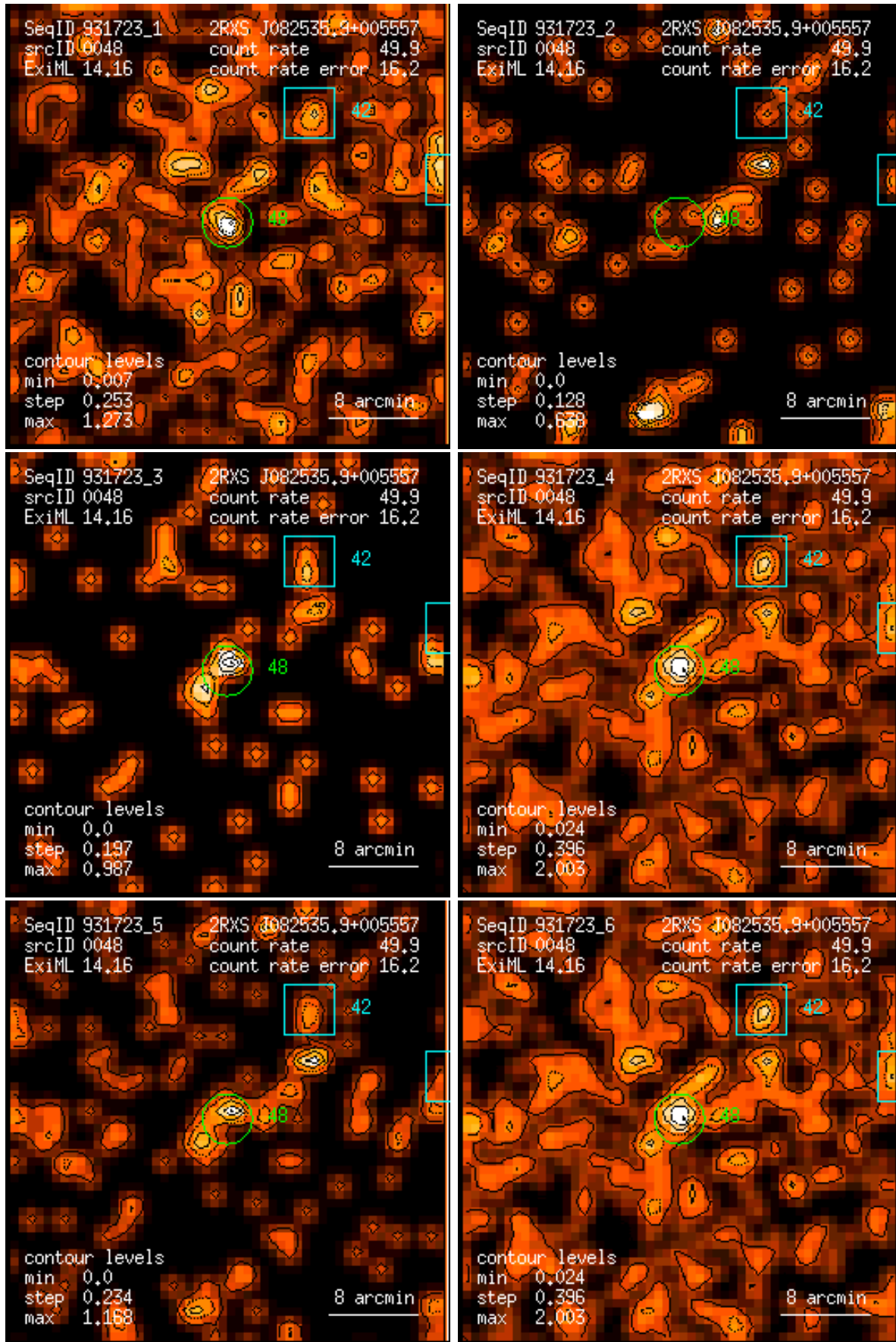
Figure 48: RASS 931723: detection 0048: band rate images, Gaussian filter: (1) PSPC channels 11 – 41, (2) 52 – 90, (3) 91 – 201, (4) 11 – 235, (5) 52 – 201, (6) 11 – 201. Broad band rates in counts/ks. Band rate contour levels in counts/ks/arcmin 2 .
