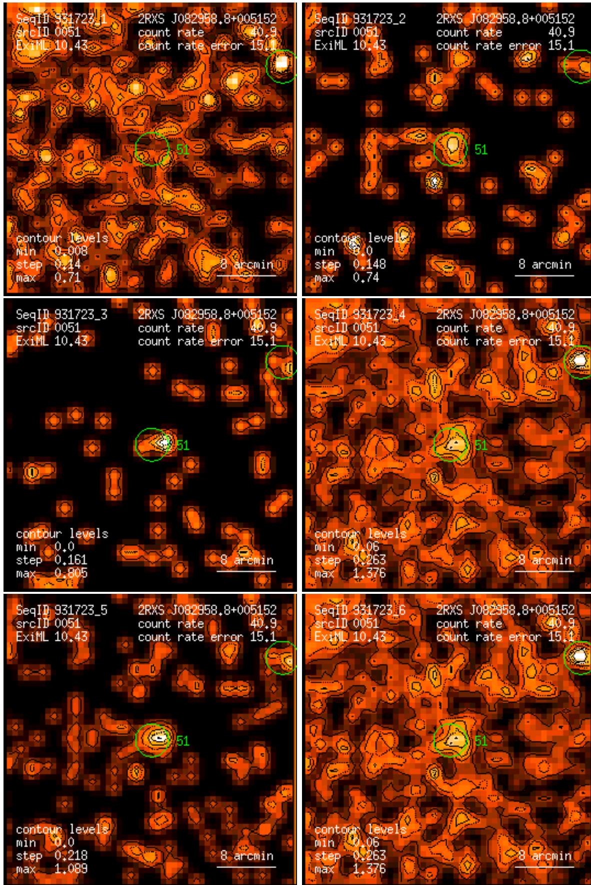
Figure 51: RASS 931723: detection 0051: band rate images, Gaussian filter: (1) PSPC channels 11 – 41, (2) 52 – 90, (3) 91 – 201, (4) 11 – 235, (5) 52 – 201, (6) 11 – 201. Broad band rates in counts/ks. Band rate contour levels in counts/ks/arcmin 2 .
