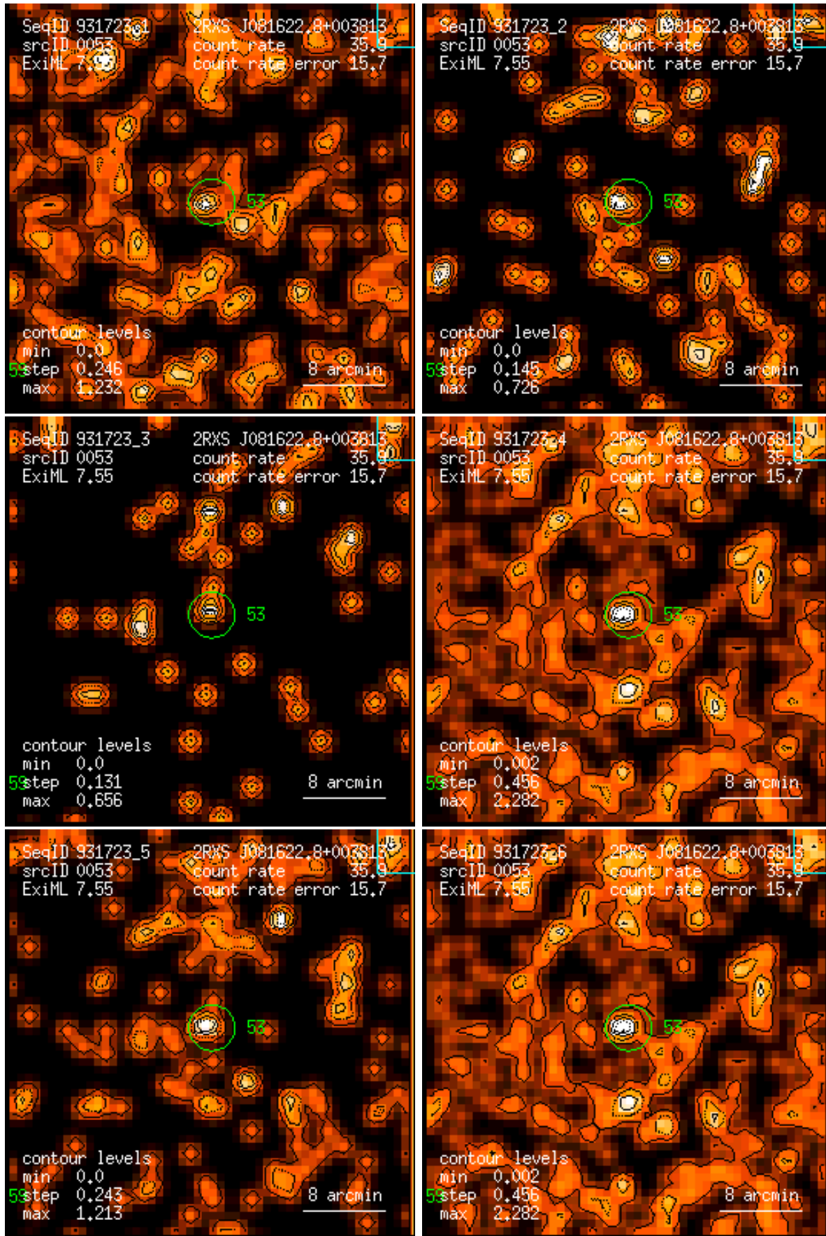
Figure 53: RASS 931723: detection 0053: band rate images, Gaussian filter: (1) PSPC channels 11 – 41, (2) 52 – 90, (3) 91 – 201, (4) 11 – 235, (5) 52 – 201, (6) 11 – 201. Broad band rates in counts/ks. Band rate contour levels in counts/ks/arcmin 2 .
