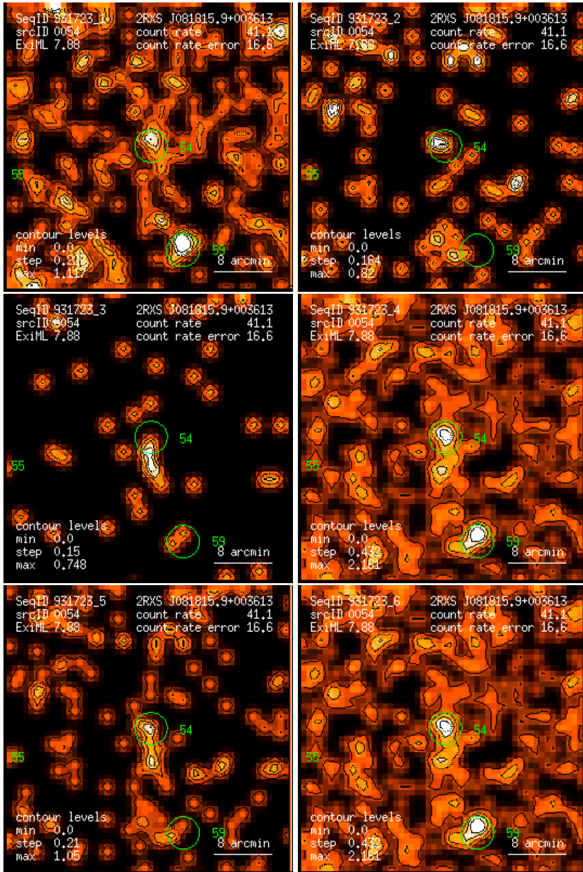
Figure 54: RASS 931723: detection 0054: band rate images, Gaussian filter: (1) PSPC channels 11 – 41, (2) 52 – 90, (3) 91 – 201, (4) 11 – 235, (5) 52 – 201, (6) 11 – 201. Broad band rates in counts/ks. Band rate contour levels in counts/ks/arcmin 2 .
