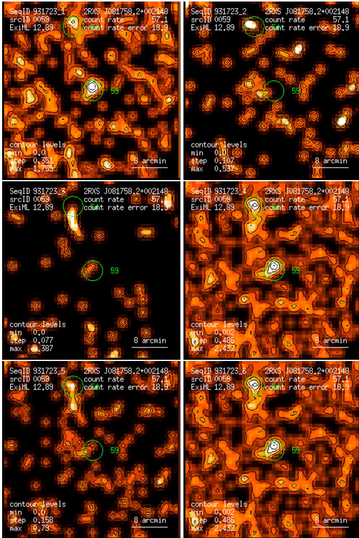
Figure 59: RASS 931723: detection 0059: band rate images, Gaussian filter: (1) PSPC channels 11 – 41, (2) 52 – 90, (3) 91 – 201, (4) 11 – 235, (5) 52 – 201, (6) 11 – 201. Broad band rates in counts/ks. Band rate contour levels in counts/ks/arcmin 2 .
