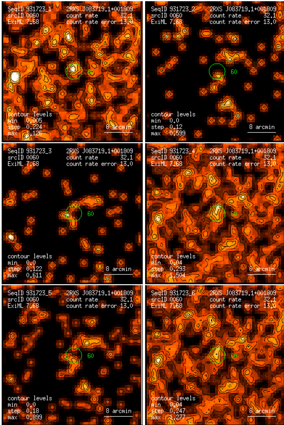
Figure 60: RASS 931723: detection 0060: band rate images, Gaussian filter: (1) PSPC channels 11 – 41, (2) 52 – 90, (3) 91 – 201, (4) 11 – 235, (5) 52 – 201, (6) 11 – 201. Broad band rates in counts/ks. Band rate contour levels in counts/ks/arcmin 2 .
