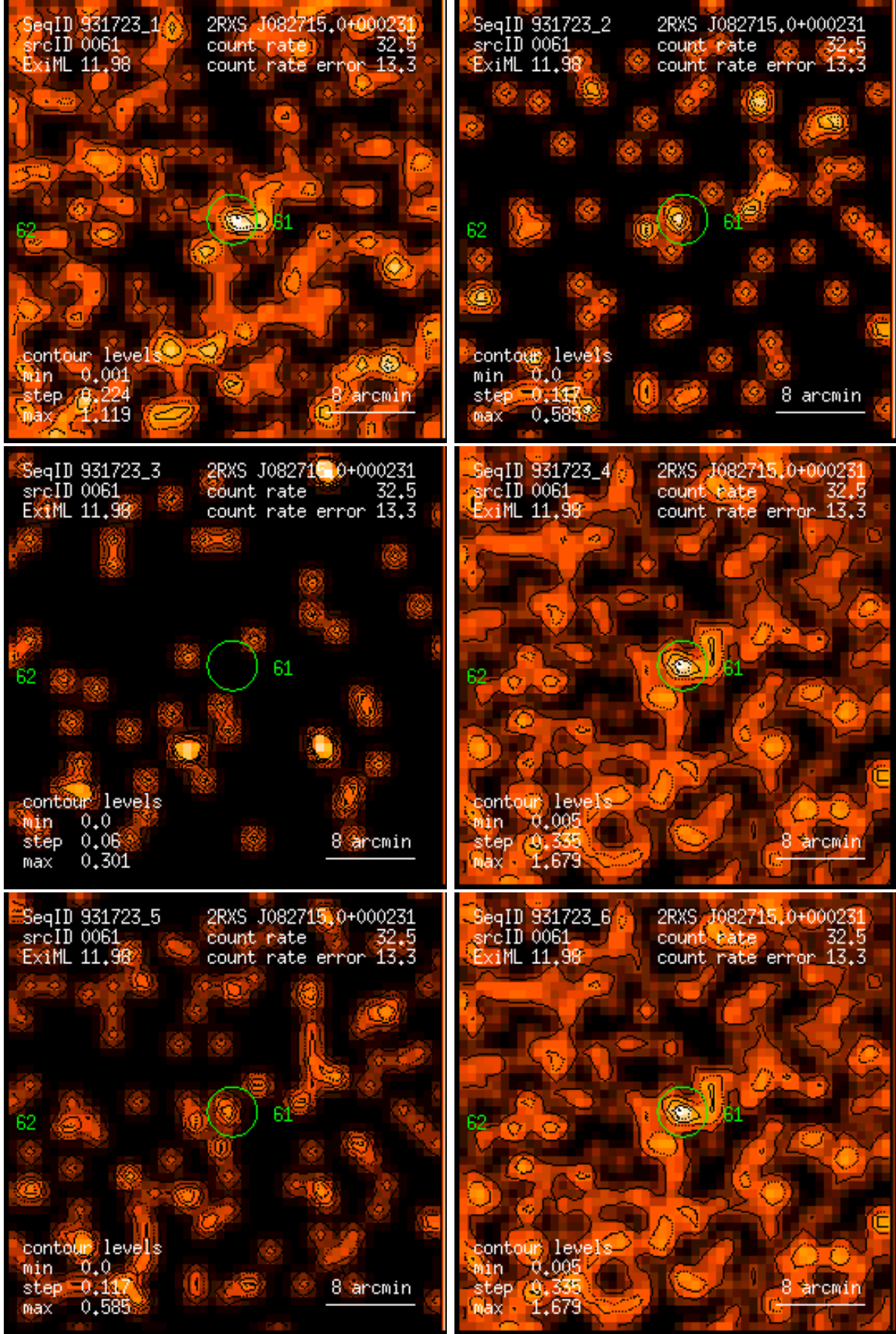
Figure 61: RASS 931723: detection 0061: band rate images, Gaussian filter: (1) PSPC channels 11 – 41, (2) 52 – 90, (3) 91 – 201, (4) 11 – 235, (5) 52 – 201, (6) 11 – 201. Broad band rates in counts/ks. Band rate contour levels in counts/ks/arcmin 2 .
