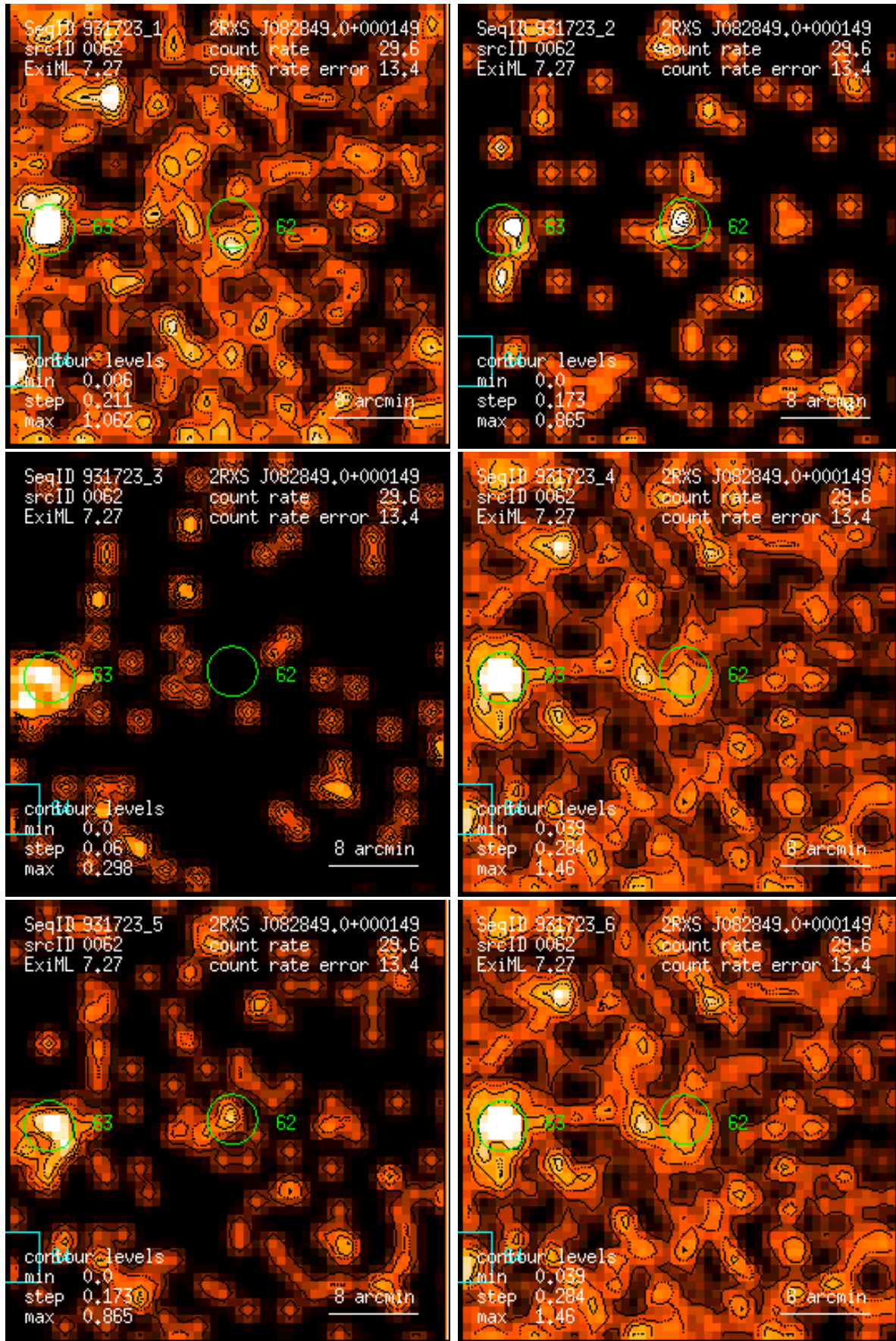
Figure 62: RASS 931723: detection 0062: band rate images, Gaussian filter: (1) PSPC channels 11 – 41, (2) 52 – 90, (3) 91 – 201, (4) 11 – 235, (5) 52 – 201, (6) 11 – 201. Broad band rates in counts/ks. Band rate contour levels in counts/ks/arcmin 2 .
