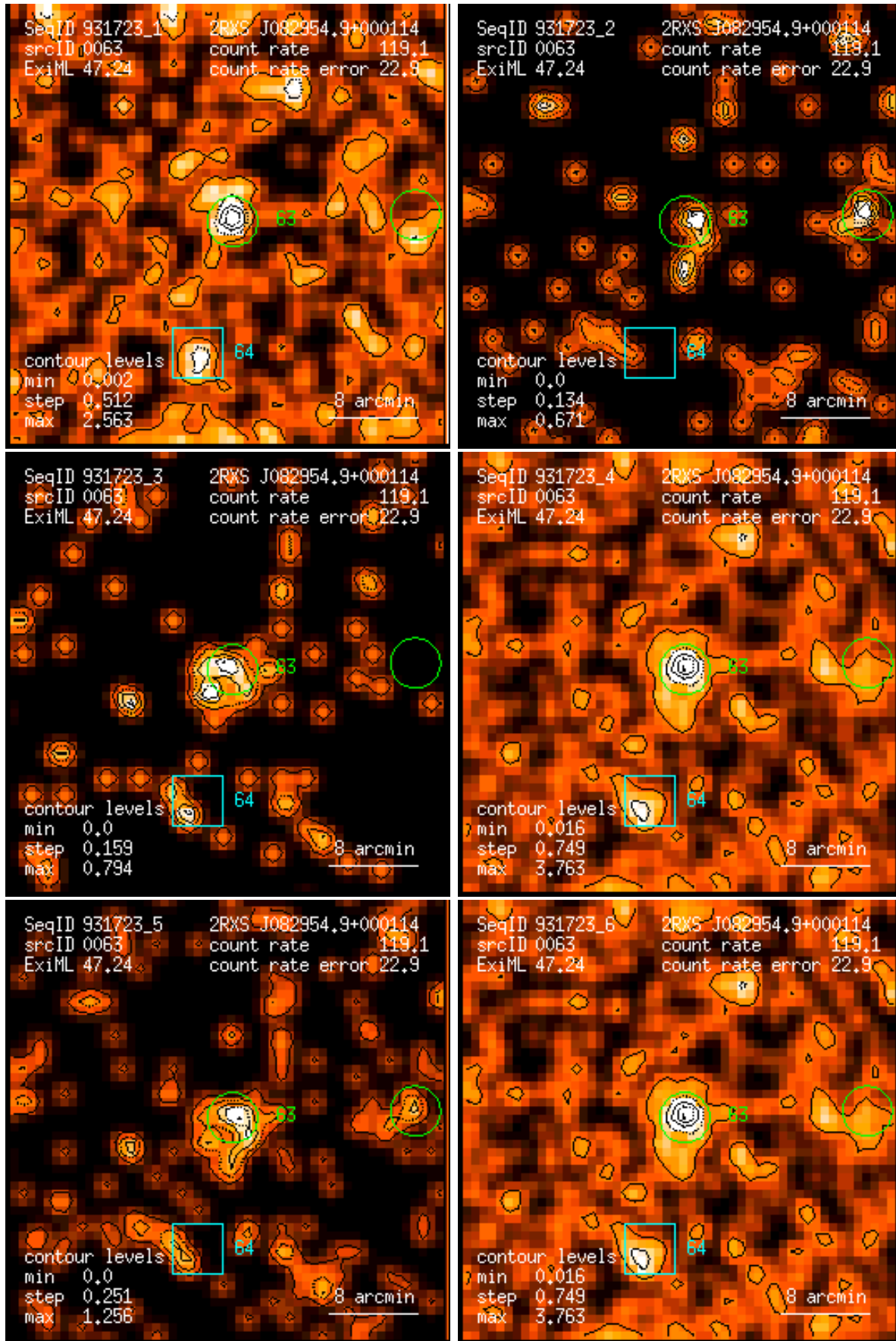
Figure 63: RASS 931723: detection 0063: band rate images, Gaussian filter: (1) PSPC channels 11 – 41, (2) 52 – 90, (3) 91 – 201, (4) 11 – 235, (5) 52 – 201, (6) 11 – 201. Broad band rates in counts/ks. Band rate contour levels in counts/ks/arcmin 2 .
