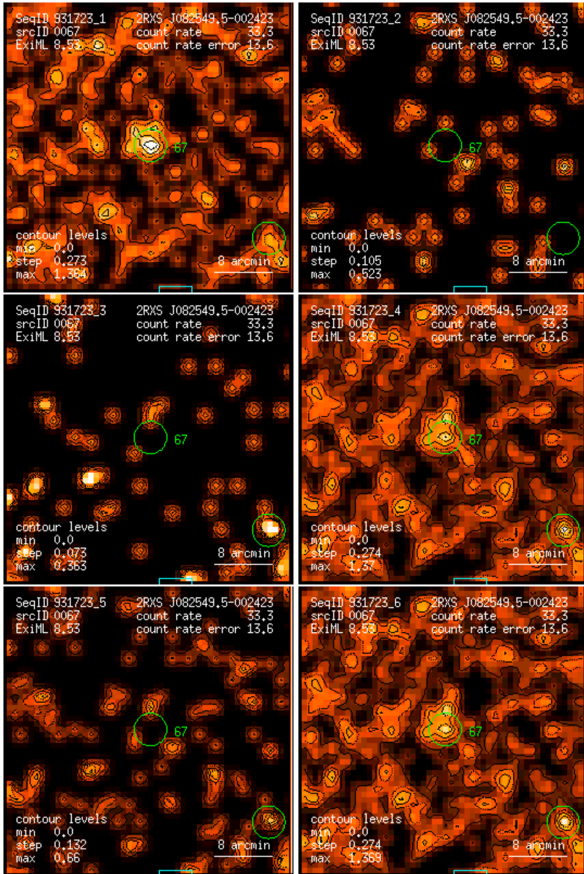
Figure 67: RASS 931723: detection 0067: band rate images, Gaussian filter: (1) PSPC channels 11 – 41, (2) 52 – 90, (3) 91 – 201, (4) 11 – 235, (5) 52 – 201, (6) 11 – 201. Broad band rates in counts/ks. Band rate contour levels in counts/ks/arcmin 2 .
