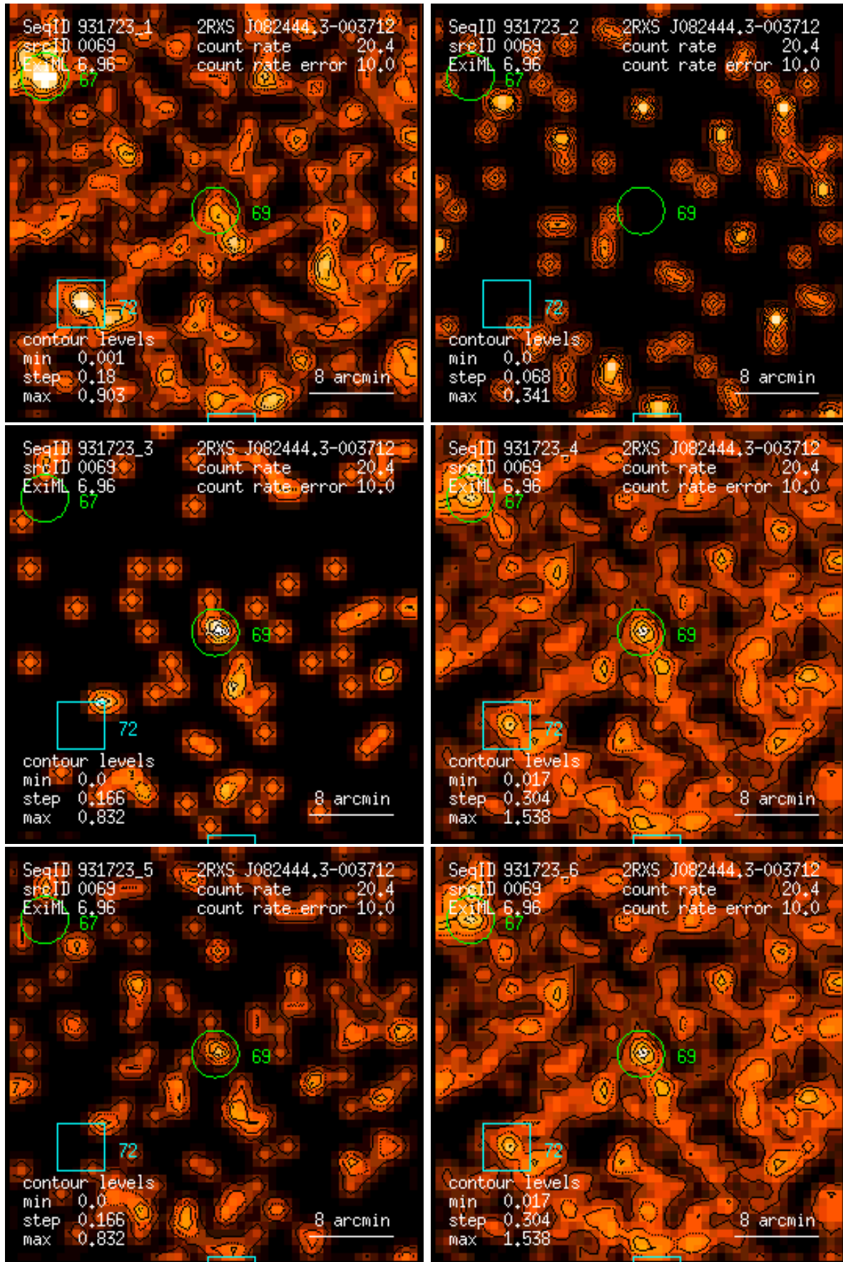
Figure 69: RASS 931723: detection 0069: band rate images, Gaussian filter: (1) PSPC channels 11 – 41, (2) 52 – 90, (3) 91 – 201, (4) 11 – 235, (5) 52 – 201, (6) 11 – 201. Broad band rates in counts/ks. Band rate contour levels in counts/ks/arcmin 2 .
