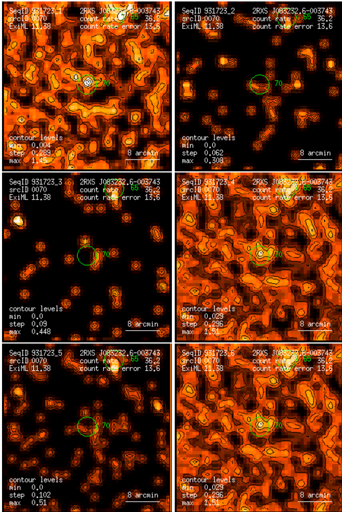
Figure 70: RASS 931723: detection 0070: band rate images, Gaussian filter: (1) PSPC channels 11 – 41, (2) 52 – 90, (3) 91 – 201, (4) 11 – 235, (5) 52 – 201, (6) 11 – 201. Broad band rates in counts/ks. Band rate contour levels in counts/ks/arcmin 2 .
