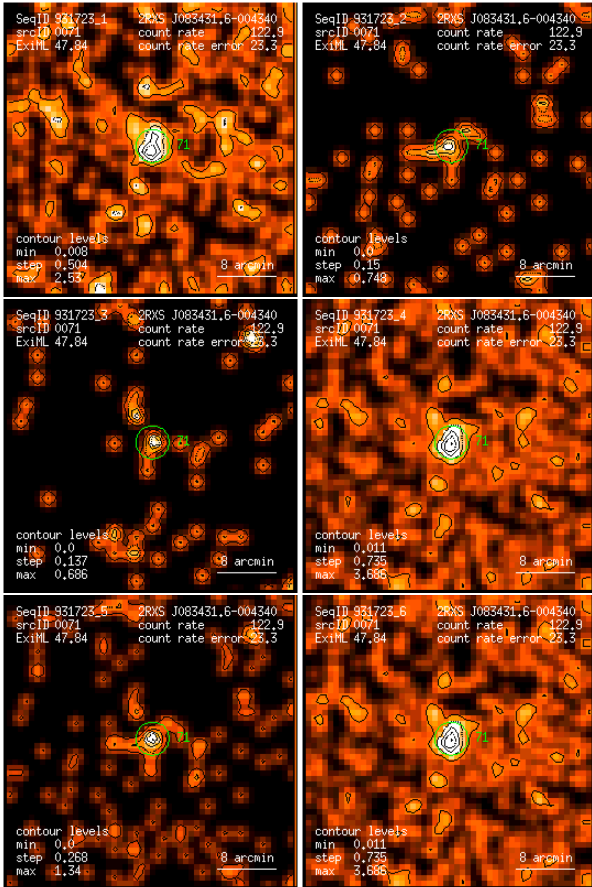
Figure 71: RASS 931723: detection 0071: band rate images, Gaussian filter: (1) PSPC channels 11 – 41, (2) 52 – 90, (3) 91 – 201, (4) 11 – 235, (5) 52 – 201, (6) 11 – 201. Broad band rates in counts/ks. Band rate contour levels in counts/ks/arcmin 2 .
