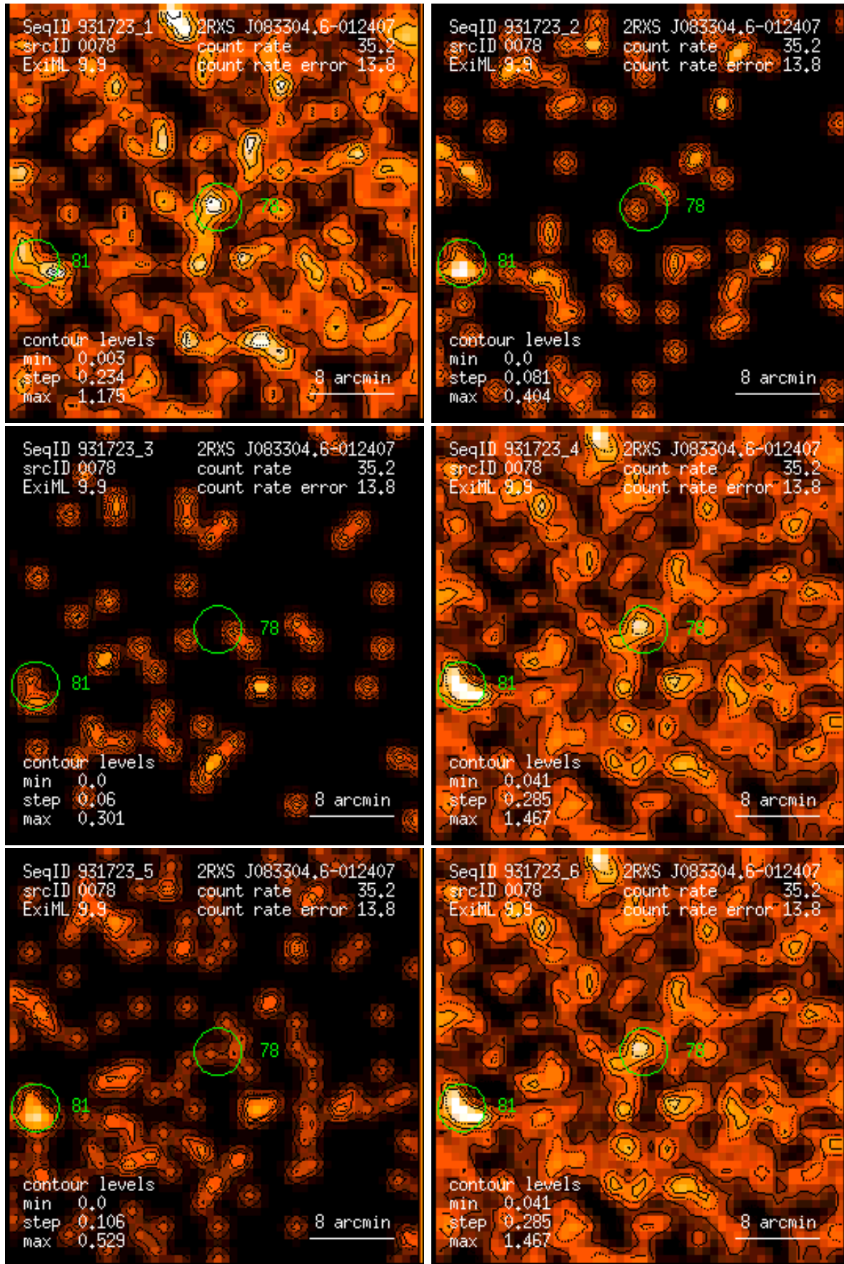
Figure 78: RASS 931723: detection 0078: band rate images, Gaussian filter: (1) PSPC channels 11 – 41, (2) 52 – 90, (3) 91 – 201, (4) 11 – 235, (5) 52 – 201, (6) 11 – 201. Broad band rates in counts/ks. Band rate contour levels in counts/ks/arcmin 2 .
