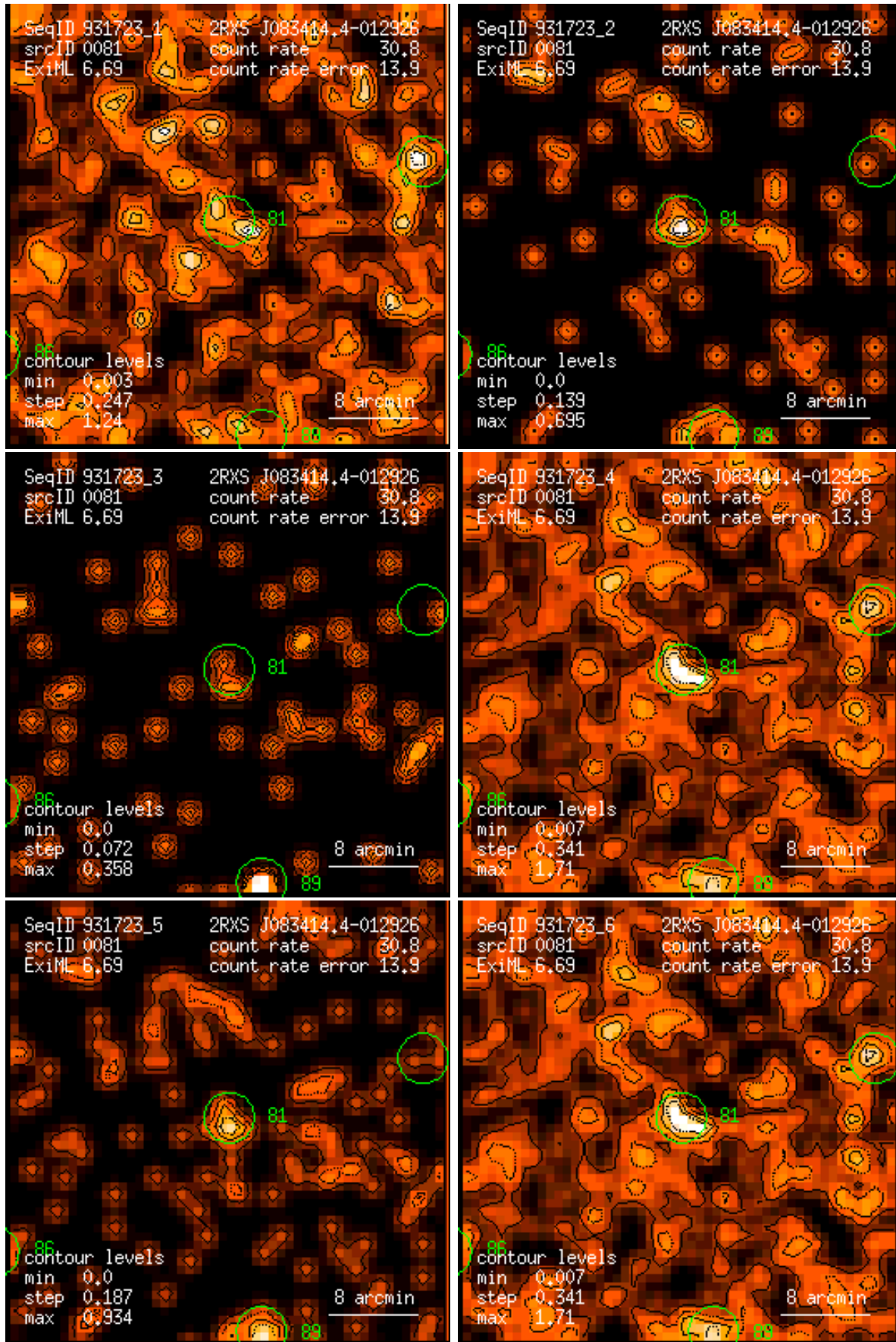
Figure 81: RASS 931723: detection 0081: band rate images, Gaussian filter: (1) PSPC channels 11 – 41, (2) 52 – 90, (3) 91 – 201, (4) 11 – 235, (5) 52 – 201, (6) 11 – 201. Broad band rates in counts/ks. Band rate contour levels in counts/ks/arcmin 2 .
