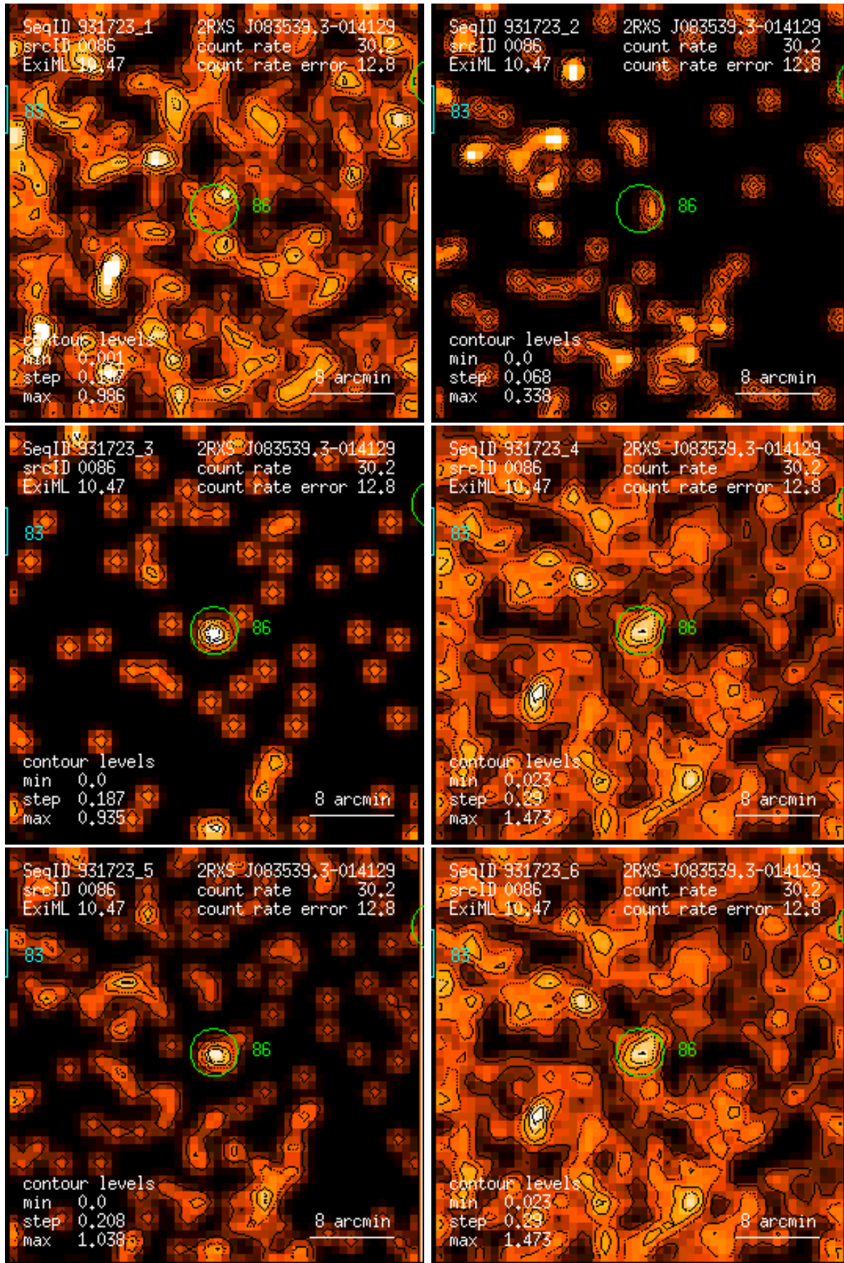
Figure 86: RASS 931723: detection 0086: band rate images, Gaussian filter: (1) PSPC channels 11 – 41, (2) 52 – 90, (3) 91 – 201, (4) 11 – 235, (5) 52 – 201, (6) 11 – 201. Broad band rates in counts/ks. Band rate contour levels in counts/ks/arcmin 2 .
