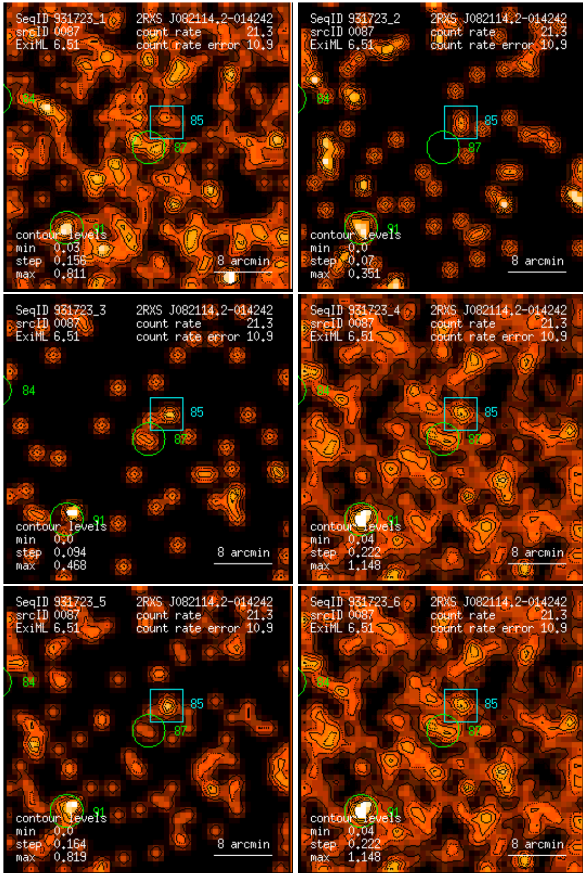
Figure 87: RASS 931723: detection 0087: band rate images, Gaussian filter: (1) PSPC channels 11 – 41, (2) 52 – 90, (3) 91 – 201, (4) 11 – 235, (5) 52 – 201, (6) 11 – 201. Broad band rates in counts/ks. Band rate contour levels in counts/ks/arcmin 2 .
