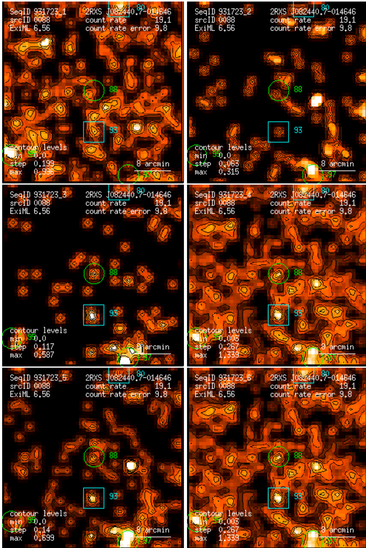
Figure 88: RASS 931723: detection 0088: band rate images, Gaussian filter: (1) PSPC channels 11 – 41, (2) 52 – 90, (3) 91 – 201, (4) 11 – 235, (5) 52 – 201, (6) 11 – 201. Broad band rates in counts/ks. Band rate contour levels in counts/ks/arcmin 2 .
