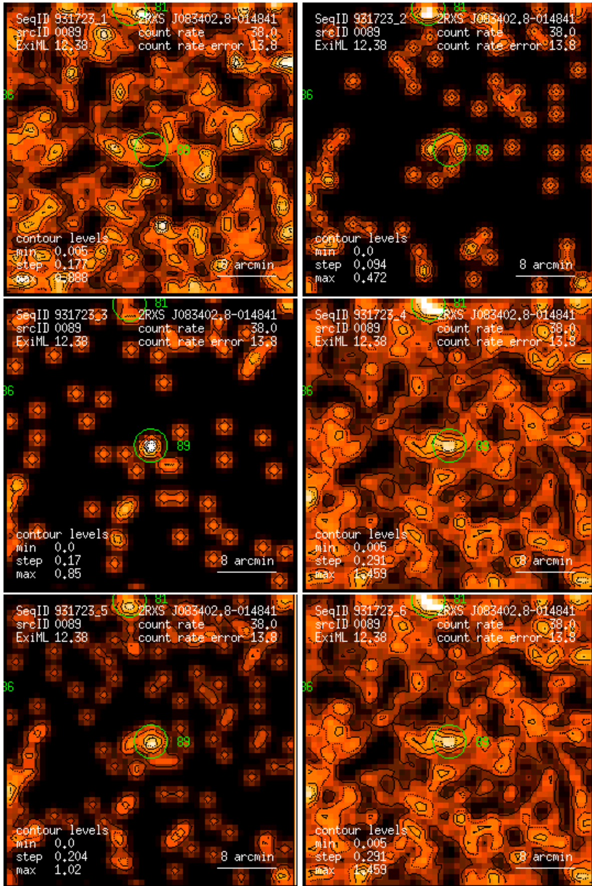
Figure 89: RASS 931723: detection 0089: band rate images, Gaussian filter: (1) PSPC channels 11 – 41, (2) 52 – 90, (3) 91 – 201, (4) 11 – 235, (5) 52 – 201, (6) 11 – 201. Broad band rates in counts/ks. Band rate contour levels in counts/ks/arcmin 2 .
