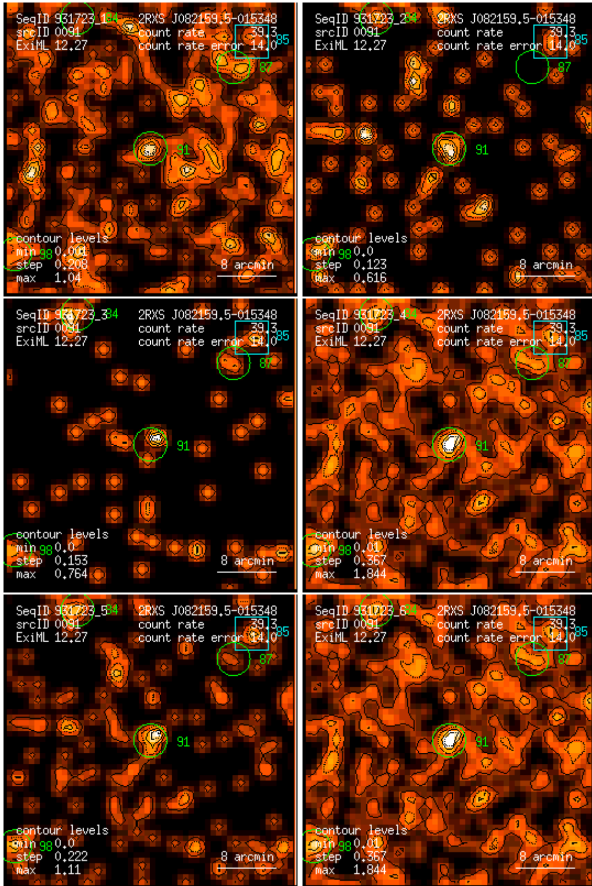
Figure 91: RASS 931723: detection 0091: band rate images, Gaussian filter: (1) PSPC channels 11 – 41, (2) 52 – 90, (3) 91 – 201, (4) 11 – 235, (5) 52 – 201, (6) 11 – 201. Broad band rates in counts/ks. Band rate contour levels in counts/ks/arcmin 2 .
