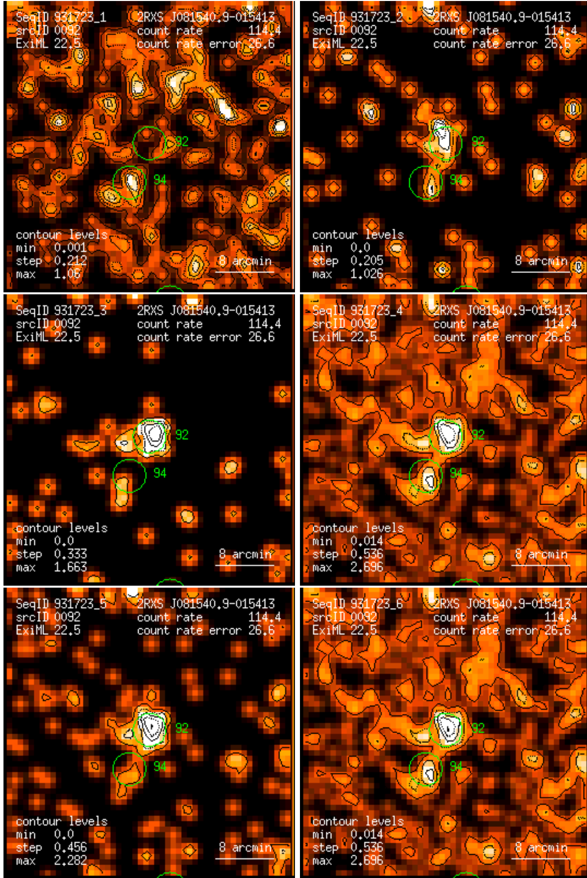
Figure 92: RASS 931723: detection 0092: band rate images, Gaussian filter: (1) PSPC channels 11 – 41, (2) 52 – 90, (3) 91 – 201, (4) 11 – 235, (5) 52 – 201, (6) 11 – 201. Broad band rates in counts/ks. Band rate contour levels in counts/ks/arcmin 2 .
