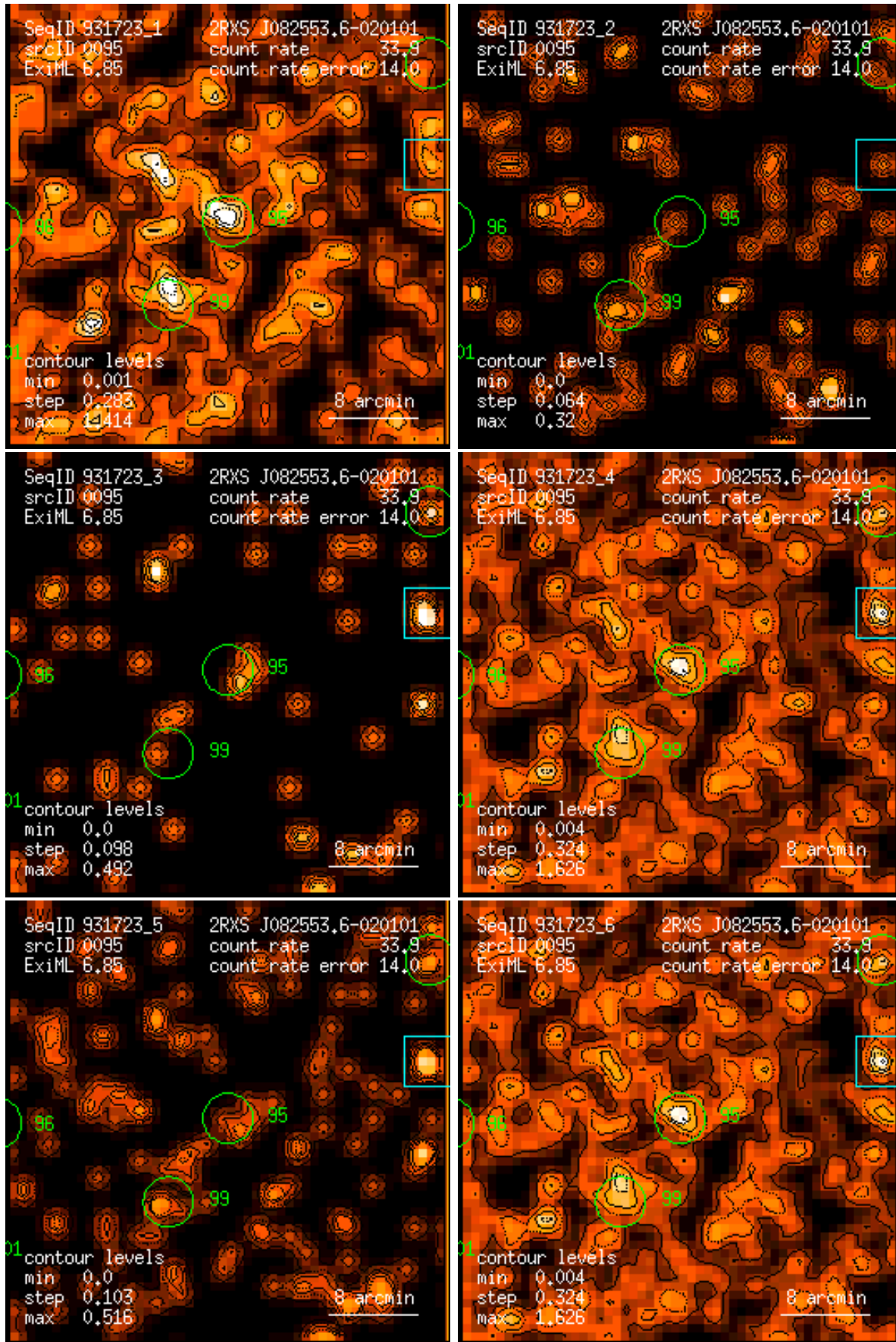
Figure 95: RASS 931723: detection 0095: band rate images, Gaussian filter: (1) PSPC channels 11 – 41, (2) 52 – 90, (3) 91 – 201, (4) 11 – 235, (5) 52 – 201, (6) 11 – 201. Broad band rates in counts/ks. Band rate contour levels in counts/ks/arcmin 2 .
