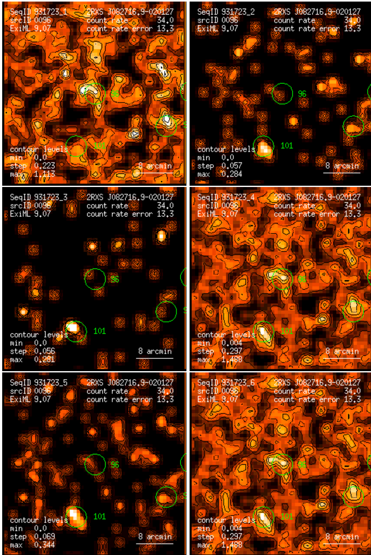
Figure 96: RASS 931723: detection 0096: band rate images, Gaussian filter: (1) PSPC channels 11 – 41, (2) 52 – 90, (3) 91 – 201, (4) 11 – 235, (5) 52 – 201, (6) 11 – 201. Broad band rates in counts/ks. Band rate contour levels in counts/ks/arcmin 2 .
