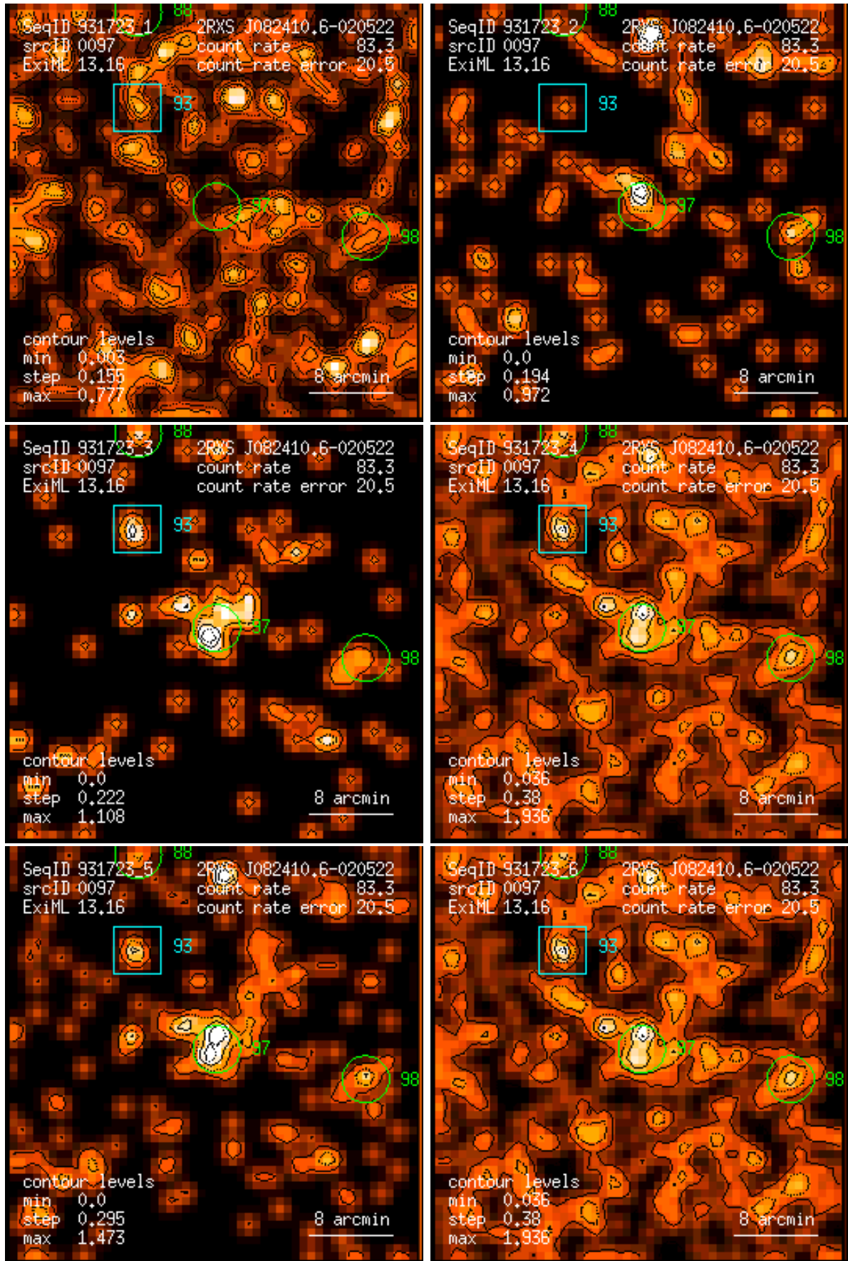
Figure 97: RASS 931723: detection 0097: band rate images, Gaussian filter: (1) PSPC channels 11 – 41, (2) 52 – 90, (3) 91 – 201, (4) 11 – 235, (5) 52 – 201, (6) 11 – 201. Broad band rates in counts/ks. Band rate contour levels in counts/ks/arcmin 2 .
