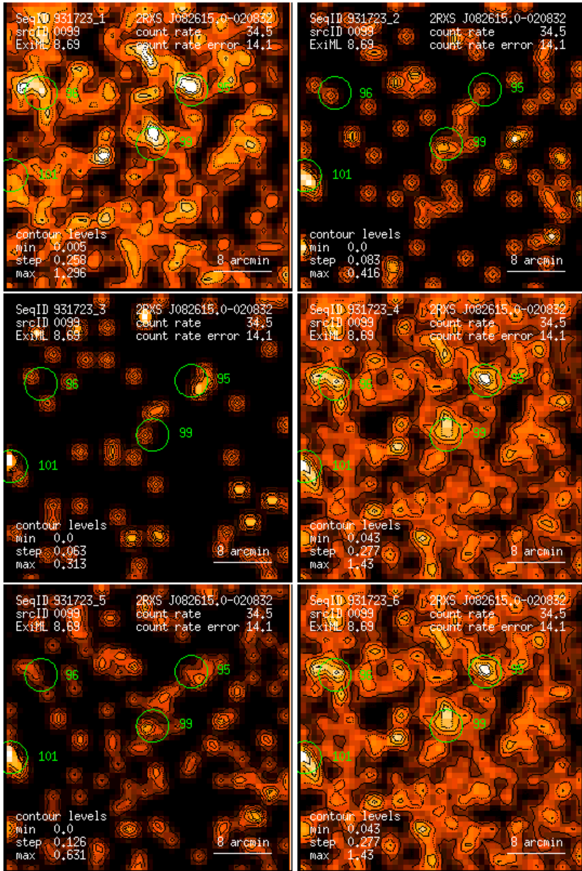
Figure 99: RASS 931723: detection 0099: band rate images, Gaussian filter: (1) PSPC channels 11 – 41, (2) 52 – 90, (3) 91 – 201, (4) 11 – 235, (5) 52 – 201, (6) 11 – 201. Broad band rates in counts/ks. Band rate contour levels in counts/ks/arcmin 2 .
