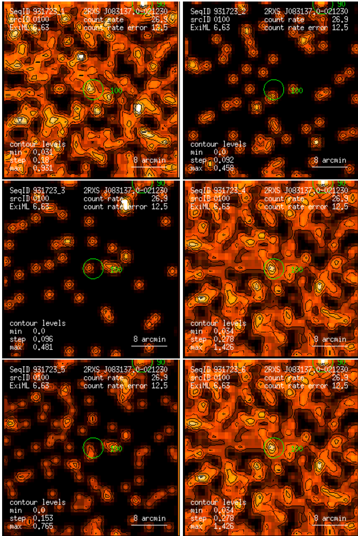
Figure 100: RASS 931723: detection 0100: band rate images, Gaussian filter: (1) PSPC channels 11 – 41, (2) 52 – 90, (3) 91 – 201, (4) 11 – 235, (5) 52 – 201, (6) 11 – 201. Broad band rates in counts/ks. Band rate contour levels in counts/ks/arcmin 2 .
