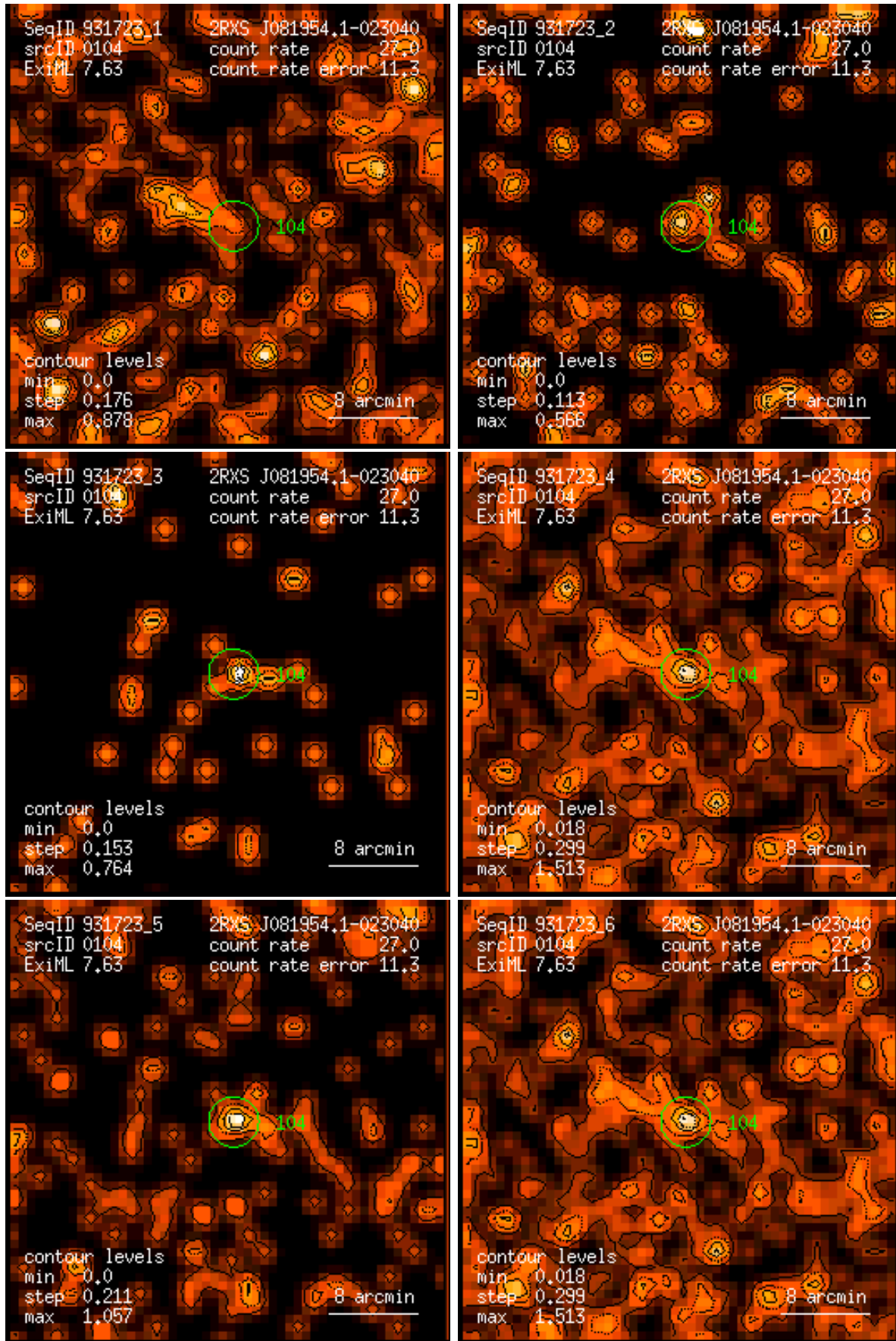
Figure 104: RASS 931723: detection 0104: band rate images, Gaussian filter: (1) PSPC channels 11 – 41, (2) 52 – 90, (3) 91 – 201, (4) 11 – 235, (5) 52 – 201, (6) 11 – 201. Broad band rates in counts/ks. Band rate contour levels in counts/ks/arcmin 2 .
