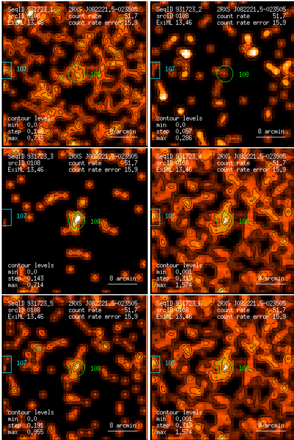
Figure 108: RASS 931723: detection 0108: band rate images, Gaussian filter: (1) PSPC channels 11 – 41, (2) 52 – 90, (3) 91 – 201, (4) 11 – 235, (5) 52 – 201, (6) 11 – 201. Broad band rates in counts/ks. Band rate contour levels in counts/ks/arcmin 2 .
