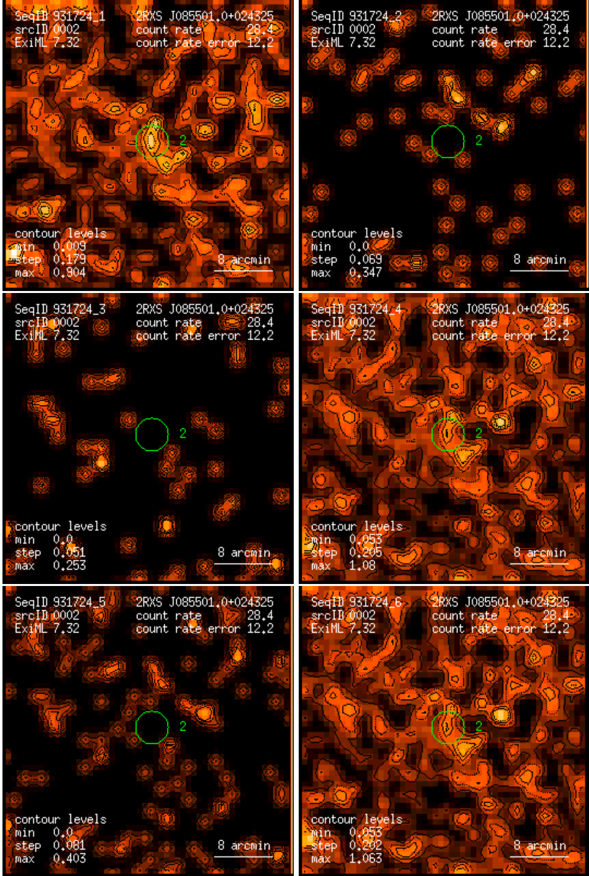
Figure 2: RASS 931724: detection 0002: band rate images, Gaussian filter: (1) PSPC channels 11 – 41, (2) 52 – 90, (3) 91 – 201, (4) 11 – 235, (5) 52 – 201, (6) 11 – 201. Broad band rates in counts/ks. Band rate contour levels in counts/ks/arcmin 2 .
