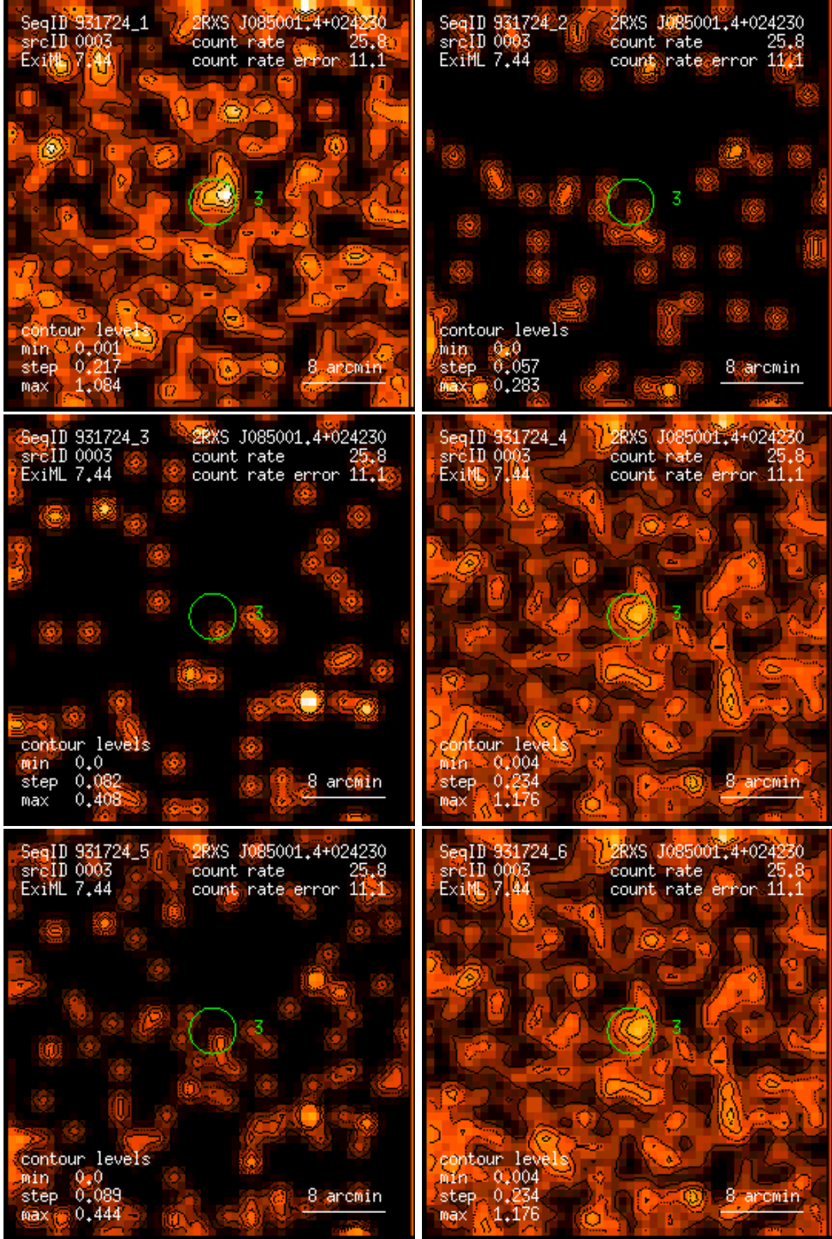
Figure 3: RASS 931724: detection 0003: band rate images, Gaussian filter: (1) PSPC channels 11 – 41, (2) 52 – 90, (3) 91 – 201, (4) 11 – 235, (5) 52 – 201, (6) 11 – 201. Broad band rates in counts/ks. Band rate contour levels in counts/ks/arcmin 2 .
