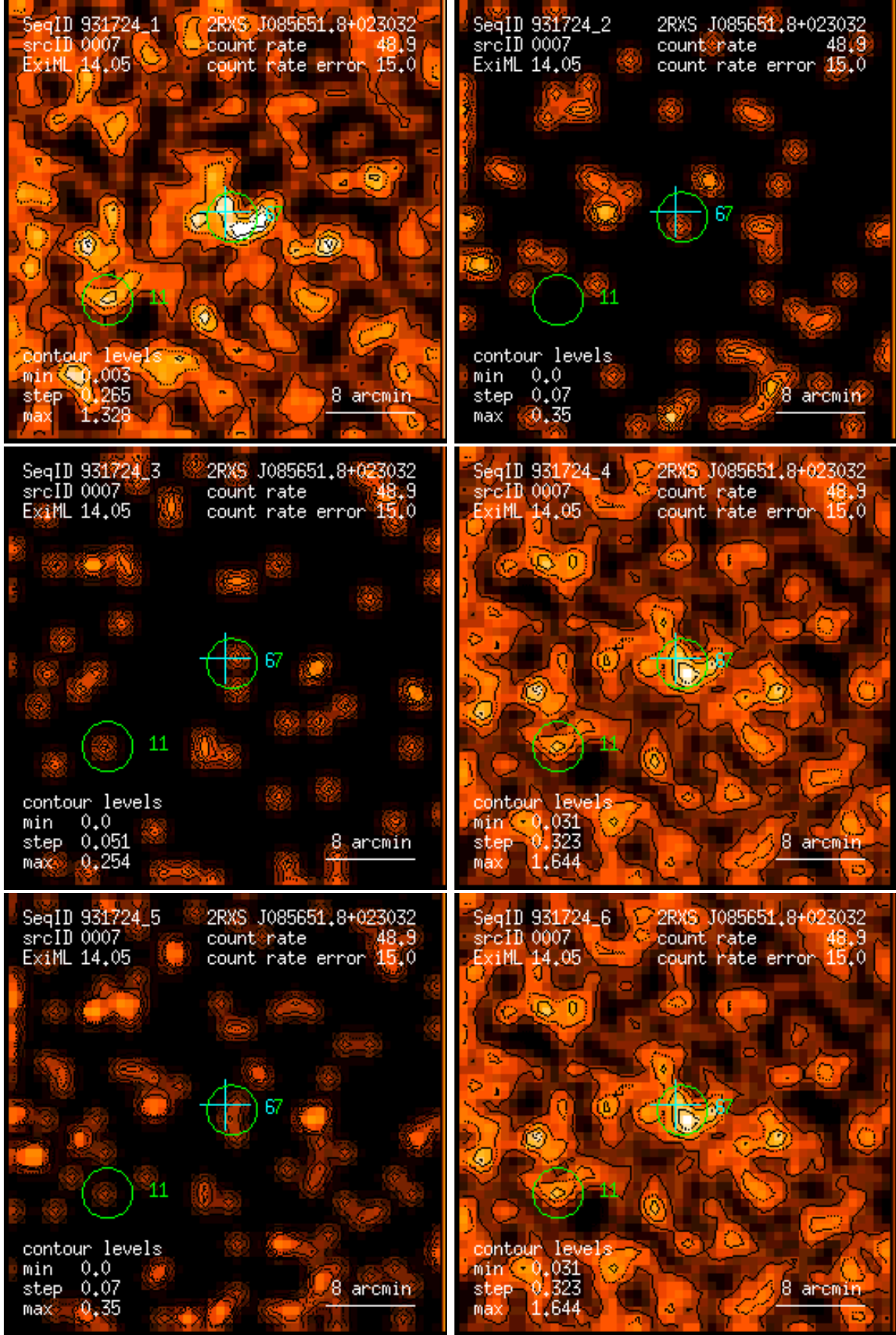
Figure 7: RASS 931724: detection 0007: band rate images, Gaussian filter: (1) PSPC channels 11 – 41, (2) 52 – 90, (3) 91 – 201, (4) 11 – 235, (5) 52 – 201, (6) 11 – 201. Broad band rates in counts/ks. Band rate contour levels in counts/ks/arcmin 2 .
