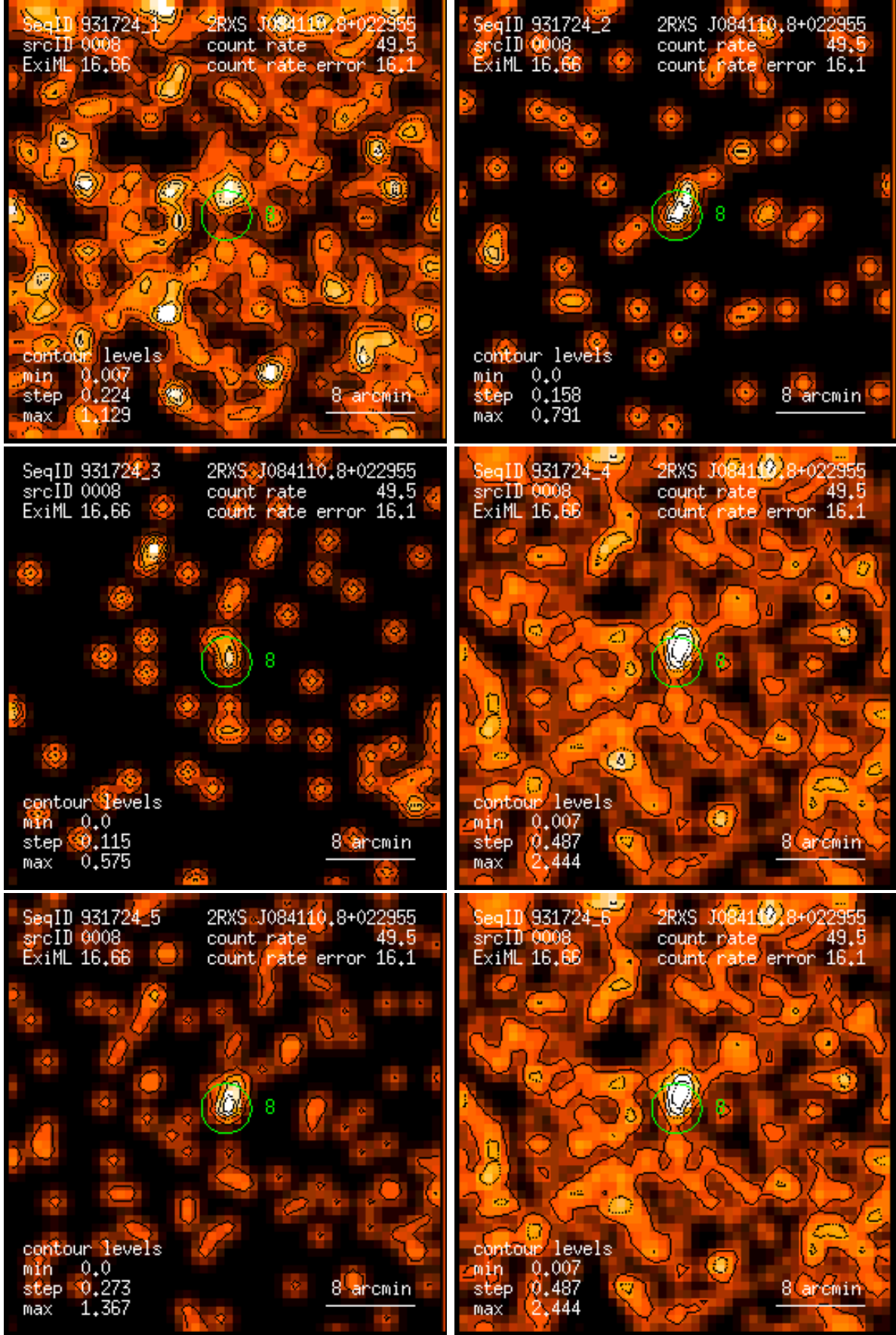
Figure 8: RASS 931724: detection 0008: band rate images, Gaussian filter: (1) PSPC channels 11 – 41, (2) 52 – 90, (3) 91 – 201, (4) 11 – 235, (5) 52 – 201, (6) 11 – 201. Broad band rates in counts/ks. Band rate contour levels in counts/ks/arcmin 2 .
