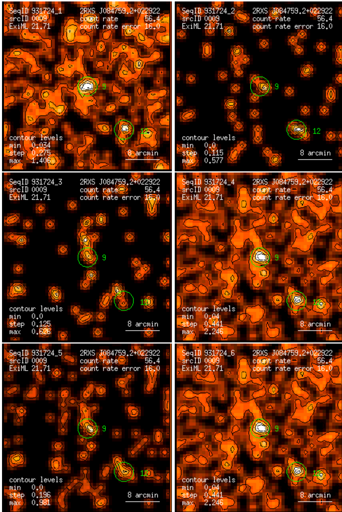
Figure 9: RASS 931724: detection 0009: band rate images, Gaussian filter: (1) PSPC channels 11 – 41, (2) 52 – 90, (3) 91 – 201, (4) 11 – 235, (5) 52 – 201, (6) 11 – 201. Broad band rates in counts/ks. Band rate contour levels in counts/ks/arcmin 2 .
