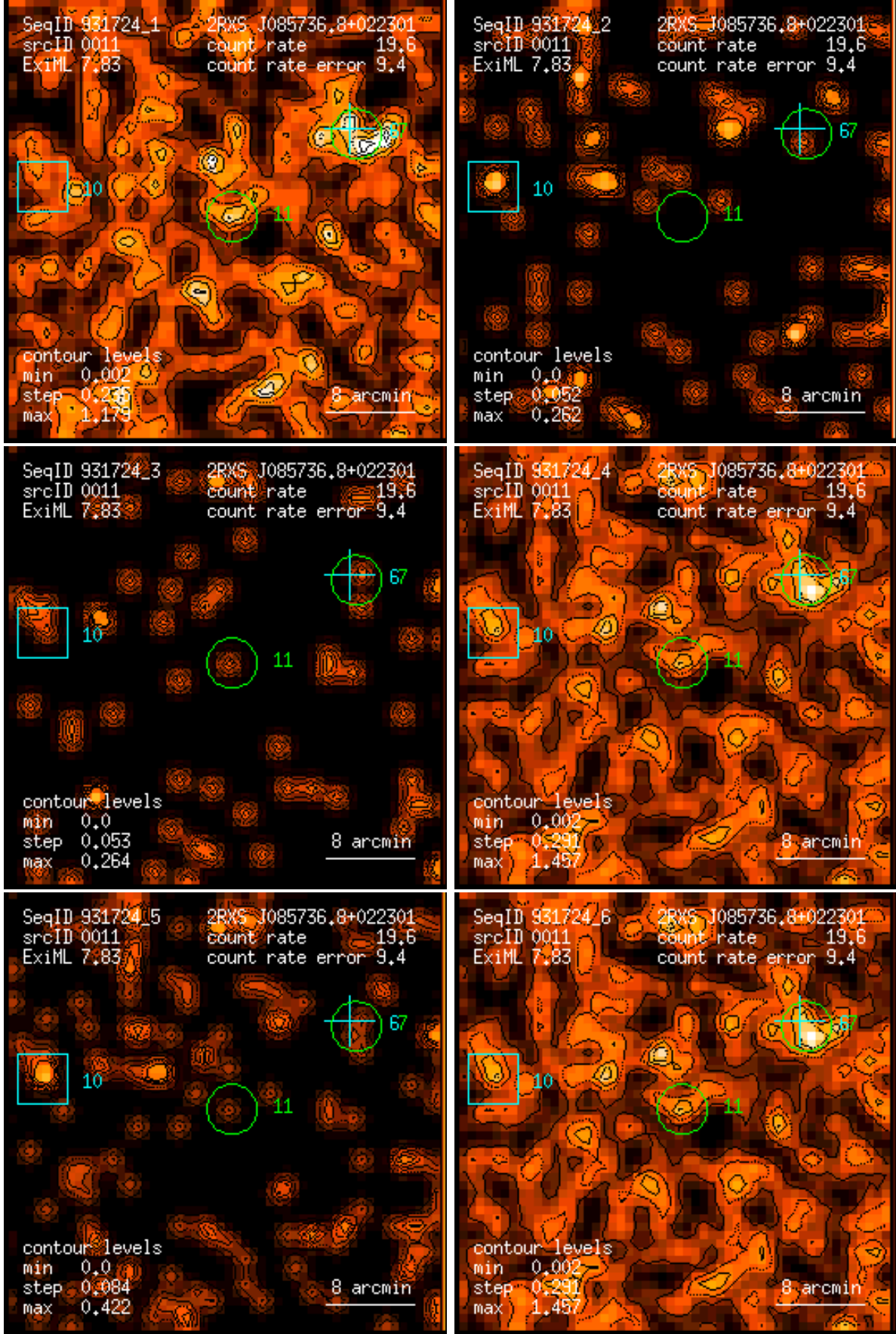
Figure 11: RASS 931724: detection 0011: band rate images, Gaussian filter: (1) PSPC channels 11 – 41, (2) 52 – 90, (3) 91 – 201, (4) 11 – 235, (5) 52 – 201, (6) 11 – 201. Broad band rates in counts/ks. Band rate contour levels in counts/ks/arcmin 2 .
