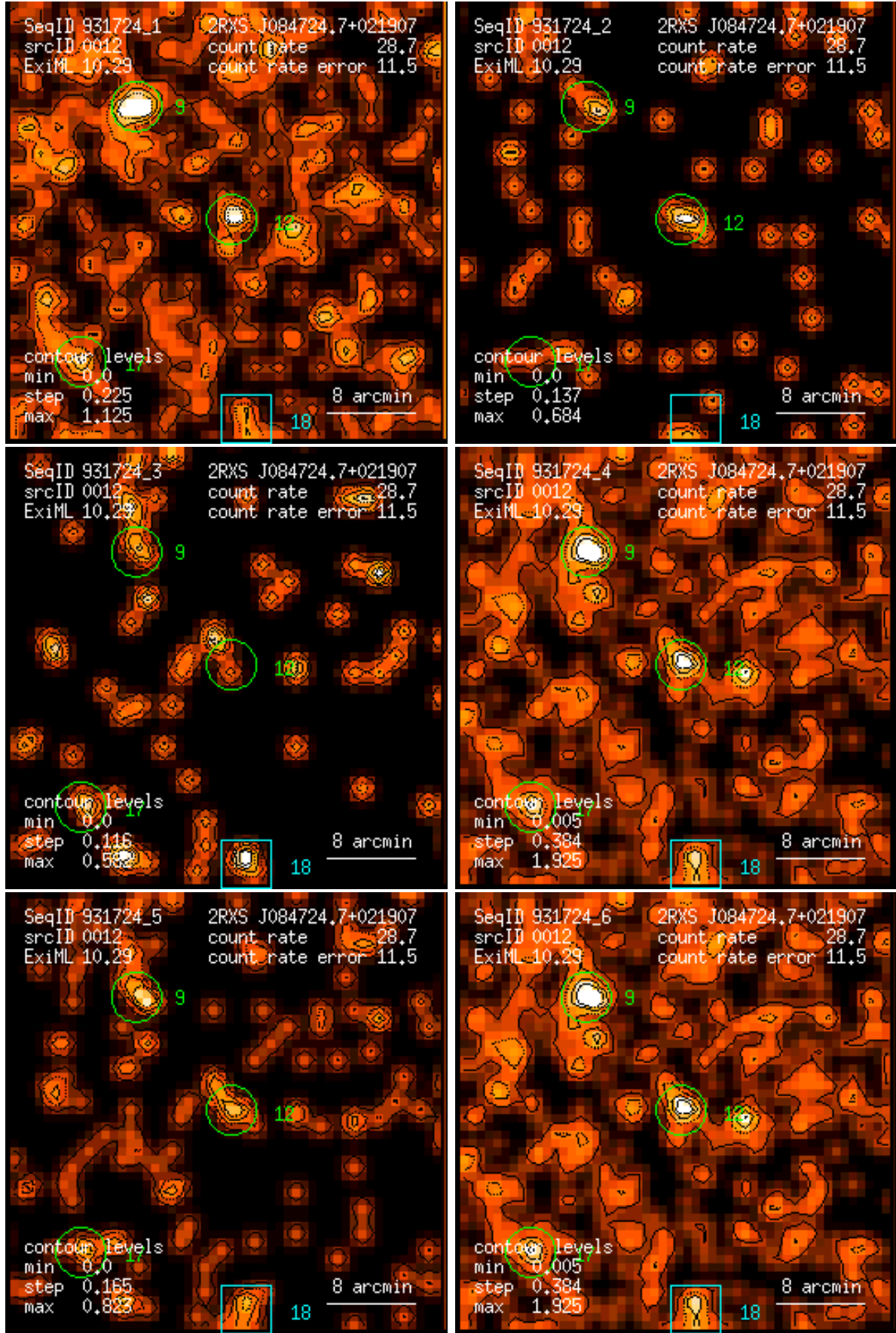
Figure 12: RASS 931724: detection 0012: band rate images, Gaussian filter: (1) PSPC channels 11 – 41, (2) 52 – 90, (3) 91 – 201, (4) 11 – 235, (5) 52 – 201, (6) 11 – 201. Broad band rates in counts/ks. Band rate contour levels in counts/ks/arcmin 2 .
