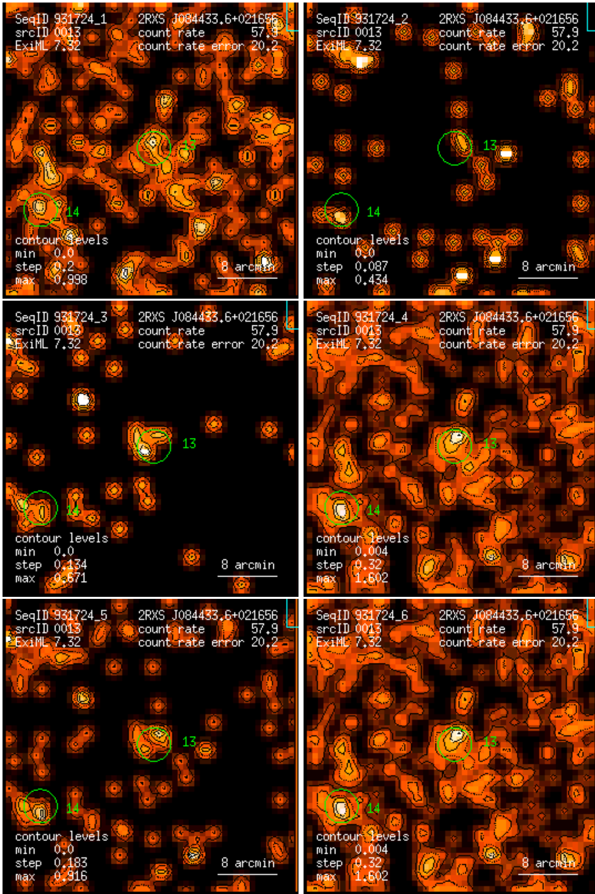
Figure 13: RASS 931724: detection 0013: band rate images, Gaussian filter: (1) PSPC channels 11 – 41, (2) 52 – 90, (3) 91 – 201, (4) 11 – 235, (5) 52 – 201, (6) 11 – 201. Broad band rates in counts/ks. Band rate contour levels in counts/ks/arcmin 2 .
