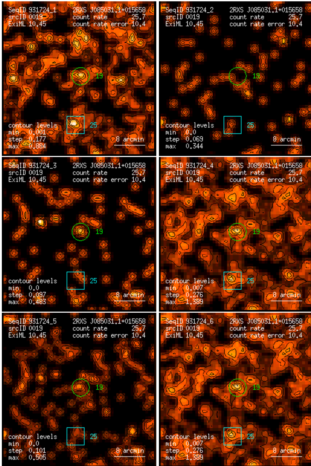
Figure 19: RASS 931724: detection 0019: band rate images, Gaussian filter: (1) PSPC channels 11 – 41, (2) 52 – 90, (3) 91 – 201, (4) 11 – 235, (5) 52 – 201, (6) 11 – 201. Broad band rates in counts/ks. Band rate contour levels in counts/ks/arcmin 2 .
