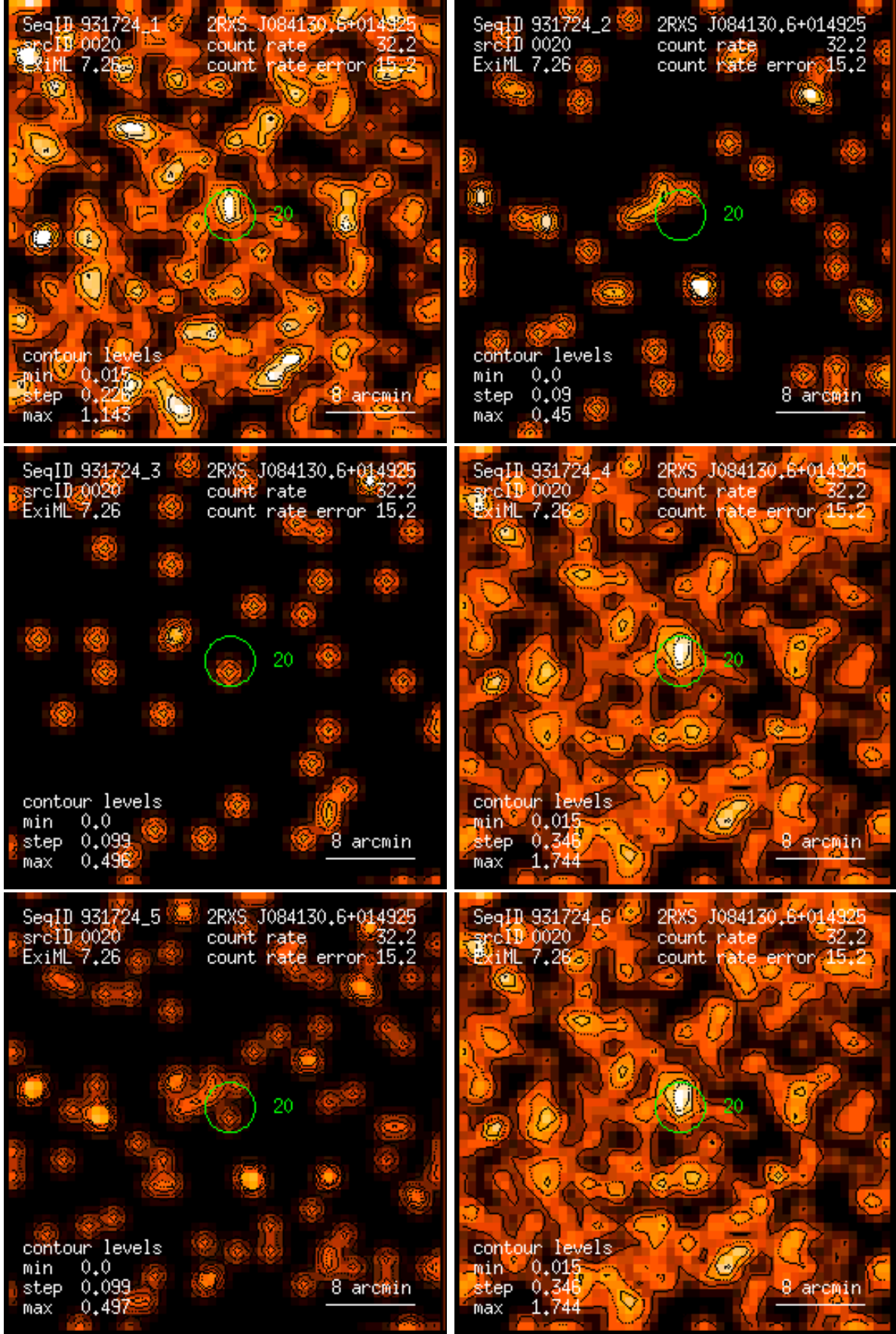
Figure 20: RASS 931724: detection 0020: band rate images, Gaussian filter: (1) PSPC channels 11 – 41, (2) 52 – 90, (3) 91 – 201, (4) 11 – 235, (5) 52 – 201, (6) 11 – 201. Broad band rates in counts/ks. Band rate contour levels in counts/ks/arcmin 2 .
