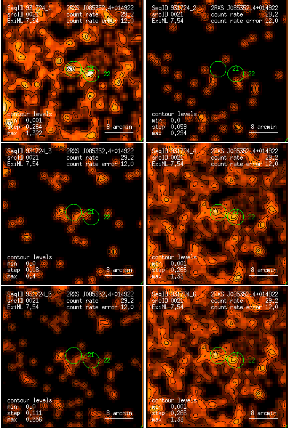
Figure 21: RASS 931724: detection 0021: band rate images, Gaussian filter: (1) PSPC channels 11 – 41, (2) 52 – 90, (3) 91 – 201, (4) 11 – 235, (5) 52 – 201, (6) 11 – 201. Broad band rates in counts/ks. Band rate contour levels in counts/ks/arcmin 2 .
