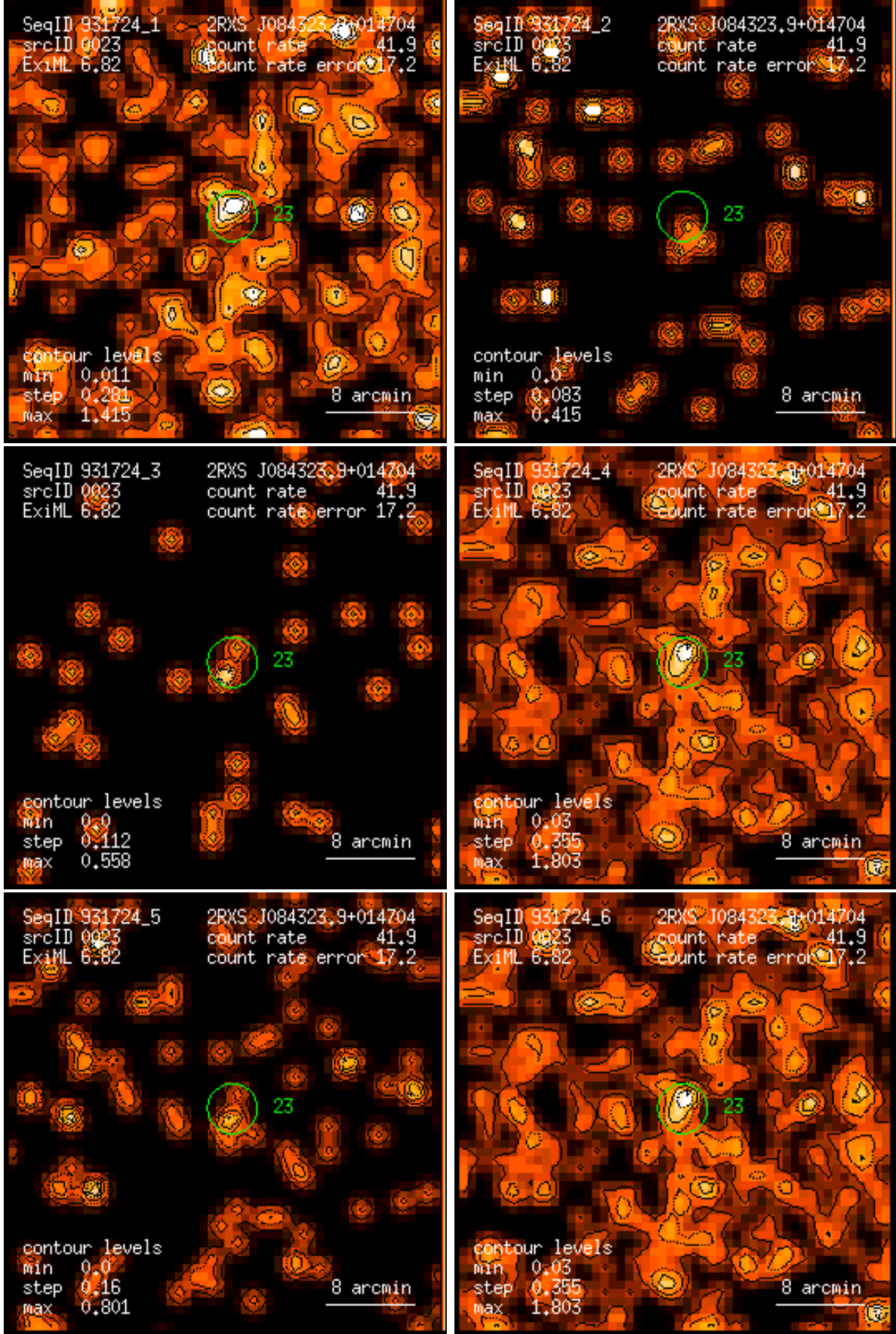
Figure 23: RASS 931724: detection 0023: band rate images, Gaussian filter: (1) PSPC channels 11 – 41, (2) 52 – 90, (3) 91 – 201, (4) 11 – 235, (5) 52 – 201, (6) 11 – 201. Broad band rates in counts/ks. Band rate contour levels in counts/ks/arcmin 2 .
