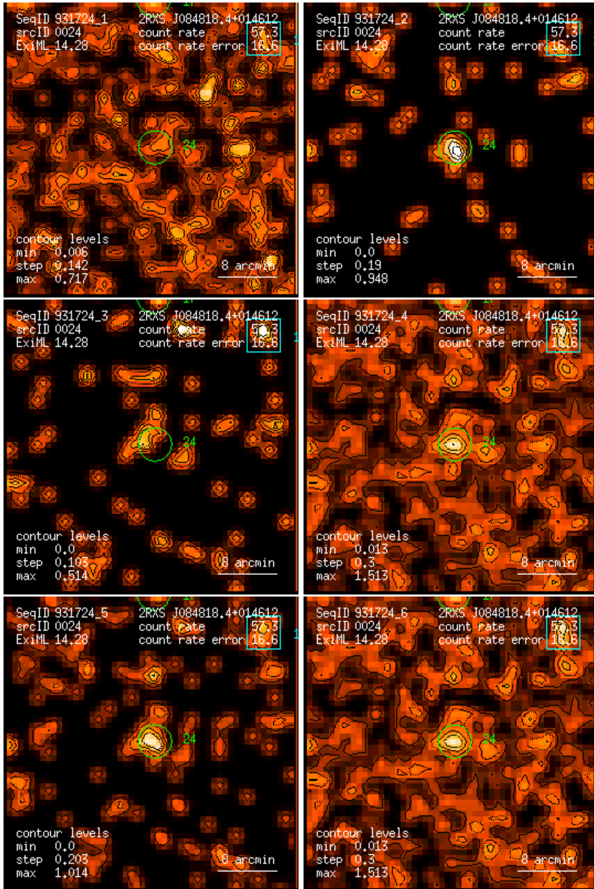
Figure 24: RASS 931724: detection 0024: band rate images, Gaussian filter: (1) PSPC channels 11 – 41, (2) 52 – 90, (3) 91 – 201, (4) 11 – 235, (5) 52 – 201, (6) 11 – 201. Broad band rates in counts/ks. Band rate contour levels in counts/ks/arcmin 2 .
