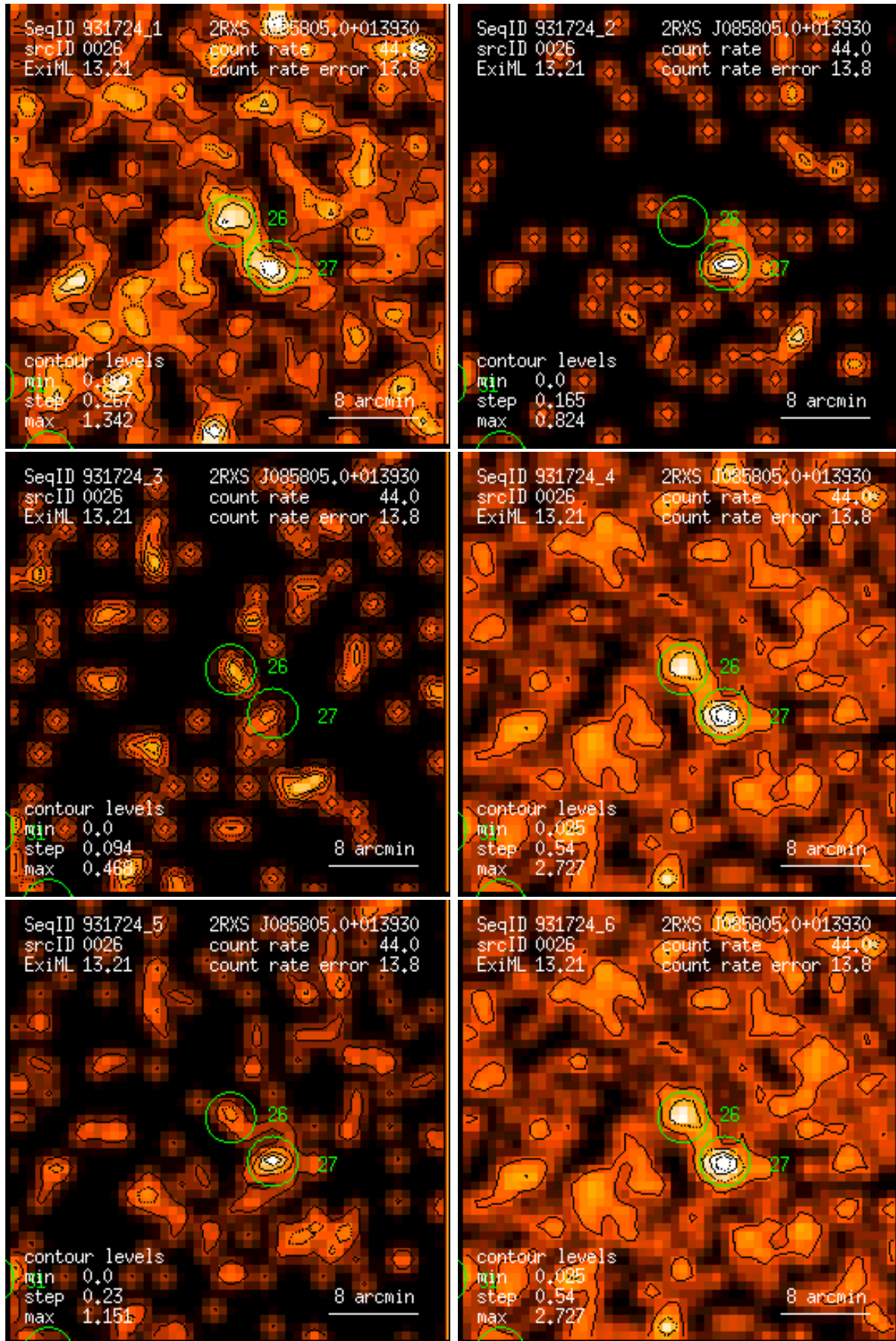
Figure 26: RASS 931724: detection 0026: band rate images, Gaussian filter: (1) PSPC channels 11 – 41, (2) 52 – 90, (3) 91 – 201, (4) 11 – 235, (5) 52 – 201, (6) 11 – 201. Broad band rates in counts/ks. Band rate contour levels in counts/ks/arcmin 2 .
