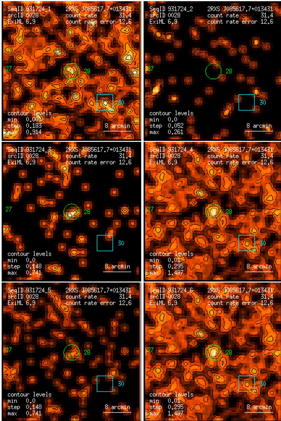
Figure 28: RASS 931724: detection 0028: band rate images, Gaussian filter: (1) PSPC channels 11 – 41, (2) 52 – 90, (3) 91 – 201, (4) 11 – 235, (5) 52 – 201, (6) 11 – 201. Broad band rates in counts/ks. Band rate contour levels in counts/ks/arcmin 2 .
