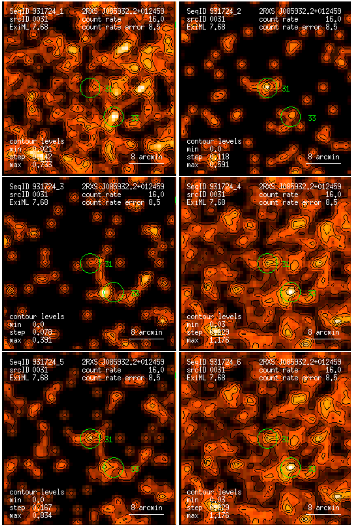
Figure 31: RASS 931724: detection 0031: band rate images, Gaussian filter: (1) PSPC channels 11 – 41, (2) 52 – 90, (3) 91 – 201, (4) 11 – 235, (5) 52 – 201, (6) 11 – 201. Broad band rates in counts/ks. Band rate contour levels in counts/ks/arcmin 2 .
