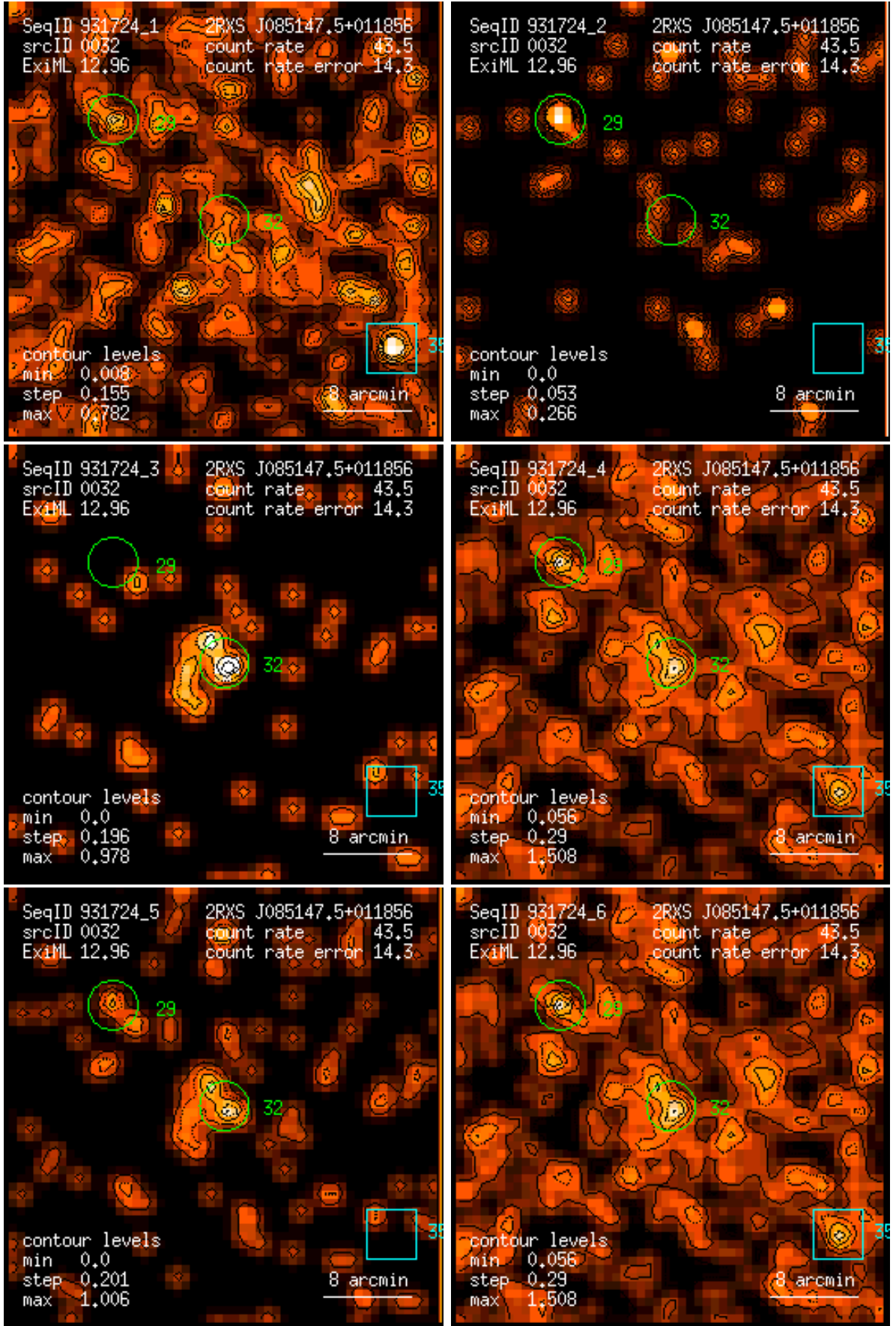
Figure 32: RASS 931724: detection 0032: band rate images, Gaussian filter: (1) PSPC channels 11 – 41, (2) 52 – 90, (3) 91 – 201, (4) 11 – 235, (5) 52 – 201, (6) 11 – 201. Broad band rates in counts/ks. Band rate contour levels in counts/ks/arcmin 2 .
