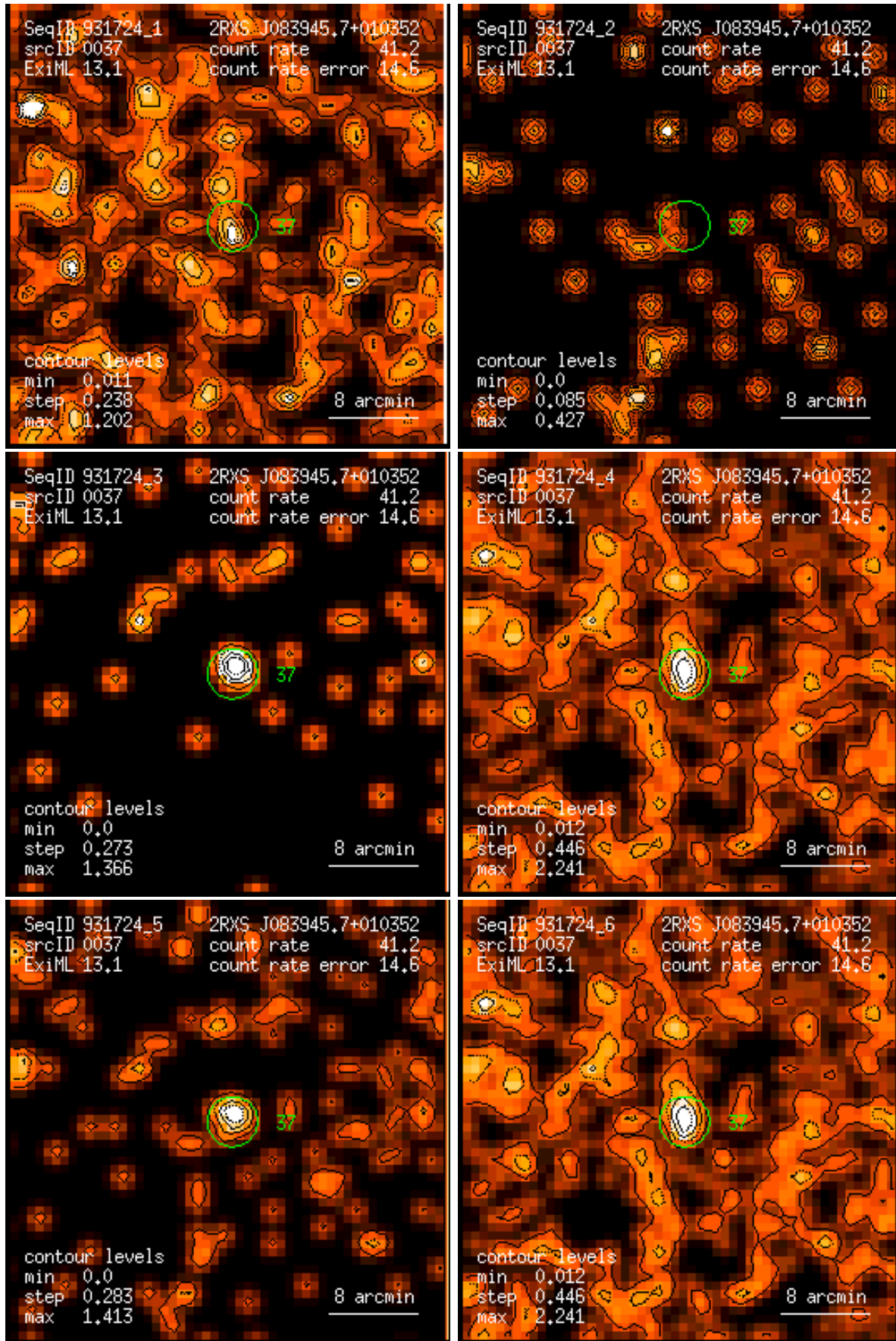
Figure 37: RASS 931724: detection 0037: band rate images, Gaussian filter: (1) PSPC channels 11 – 41, (2) 52 – 90, (3) 91 – 201, (4) 11 – 235, (5) 52 – 201, (6) 11 – 201. Broad band rates in counts/ks. Band rate contour levels in counts/ks/arcmin 2 .
