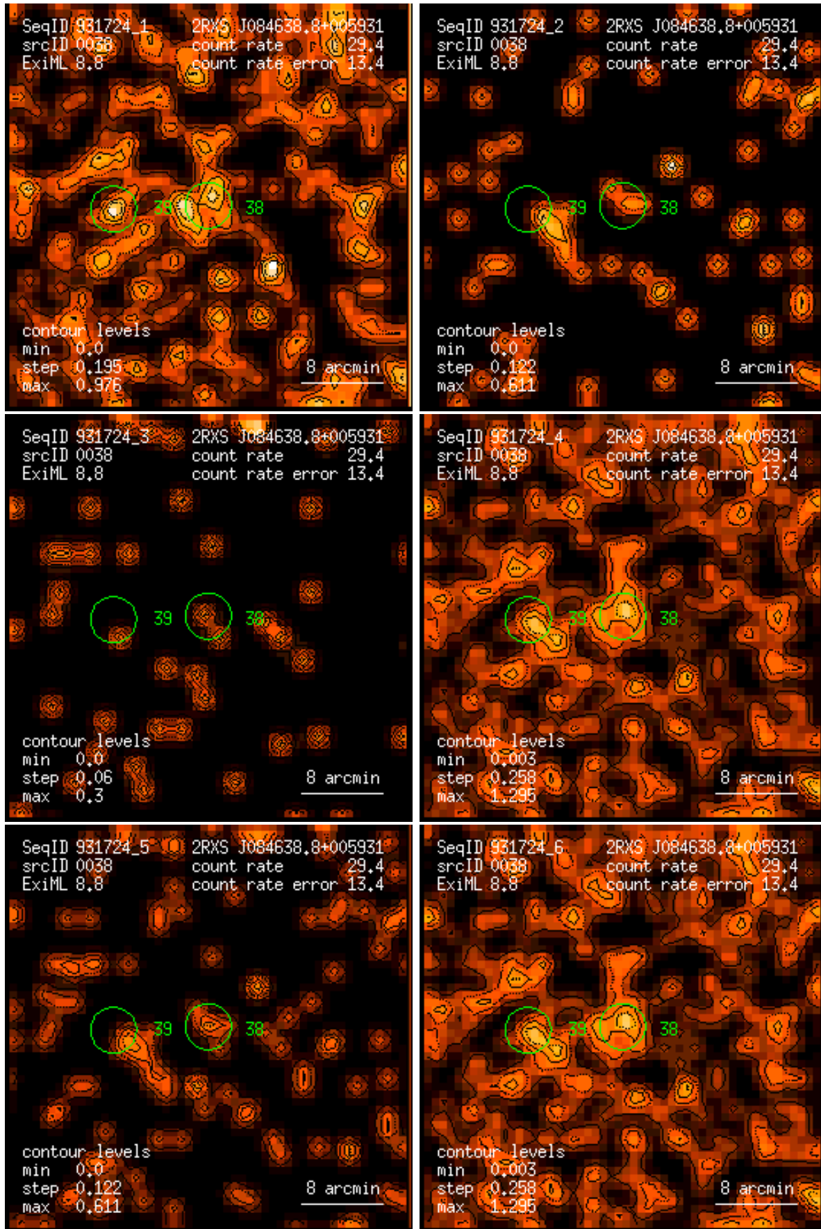
Figure 38: RASS 931724: detection 0038: band rate images, Gaussian filter: (1) PSPC channels 11 – 41, (2) 52 – 90, (3) 91 – 201, (4) 11 – 235, (5) 52 – 201, (6) 11 – 201. Broad band rates in counts/ks. Band rate contour levels in counts/ks/arcmin 2 .
