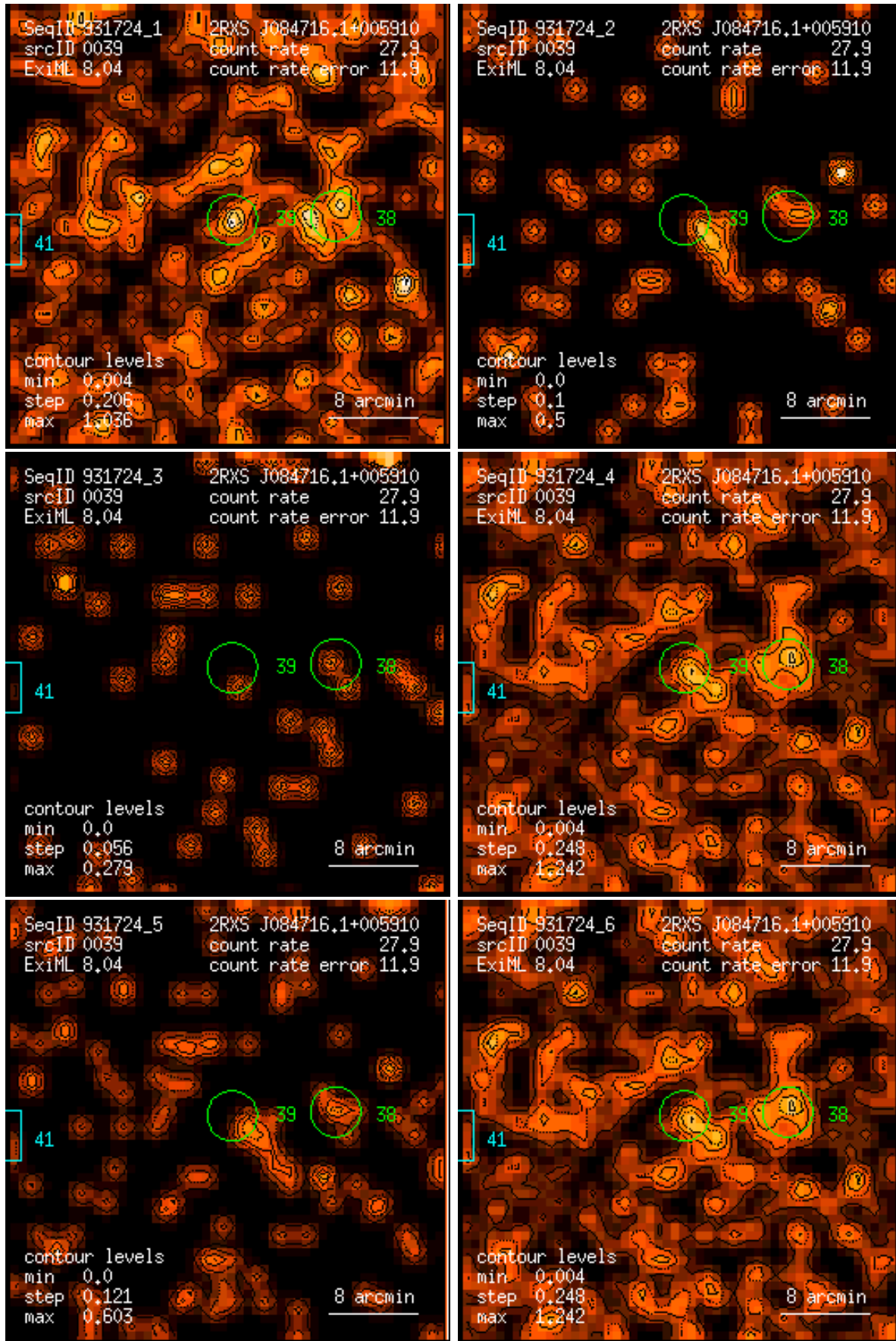
Figure 39: RASS 931724: detection 0039: band rate images, Gaussian filter: (1) PSPC channels 11 – 41, (2) 52 – 90, (3) 91 – 201, (4) 11 – 235, (5) 52 – 201, (6) 11 – 201. Broad band rates in counts/ks. Band rate contour levels in counts/ks/arcmin 2 .
