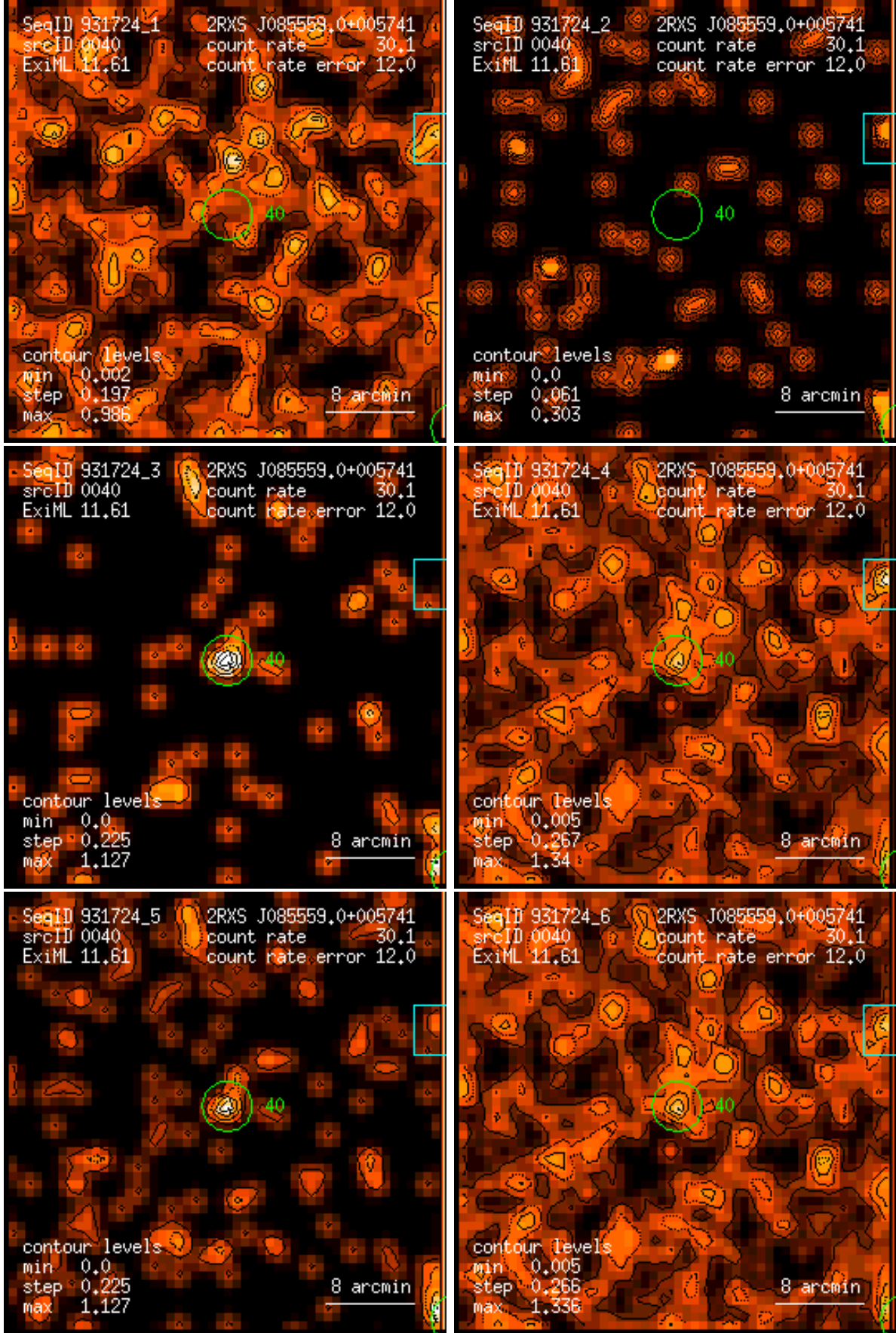
Figure 40: RASS 931724: detection 0040: band rate images, Gaussian filter: (1) PSPC channels 11 – 41, (2) 52 – 90, (3) 91 – 201, (4) 11 – 235, (5) 52 – 201, (6) 11 – 201. Broad band rates in counts/ks. Band rate contour levels in counts/ks/arcmin 2 .
